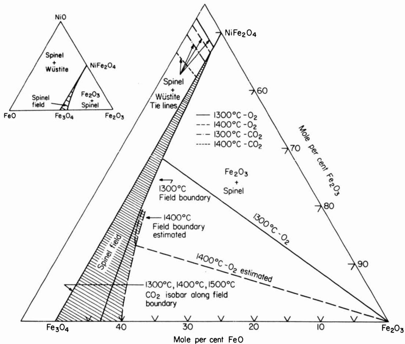
A PORTION OF THE FeO-NiO-Fe 2 O 3 PHASE DIAGRAM
