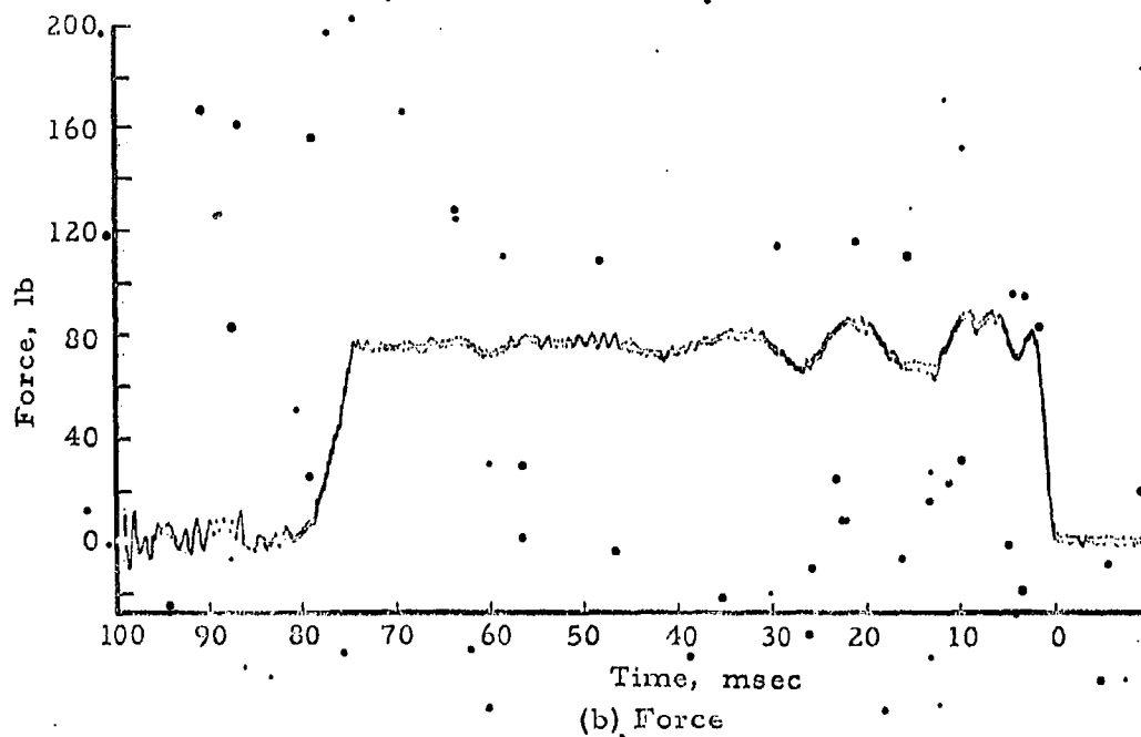
Fig. C-5 TYPICAL RECORDS FOR DYNAMICALLY LOADED FOOTING (Exper. No. P33)
