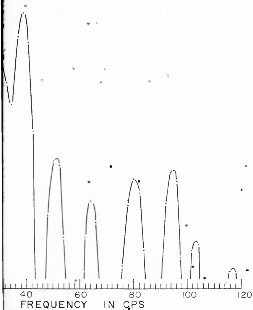
Fig. 9 Smoothed Energy Density Spectra of Signals and Power Density Spectra of the Noise Samples for the 500 pound Decoupled and Tamped Events
