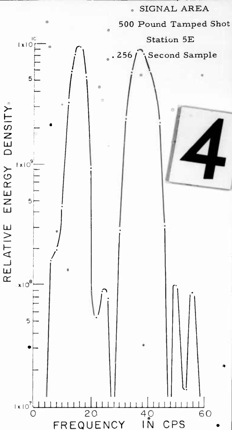
Fig. 9 Smoothed Energy Density Spectra of Signals and Power Density Spectra of the Noise Samples for the 500 pound Decoupled and Tamped Events
