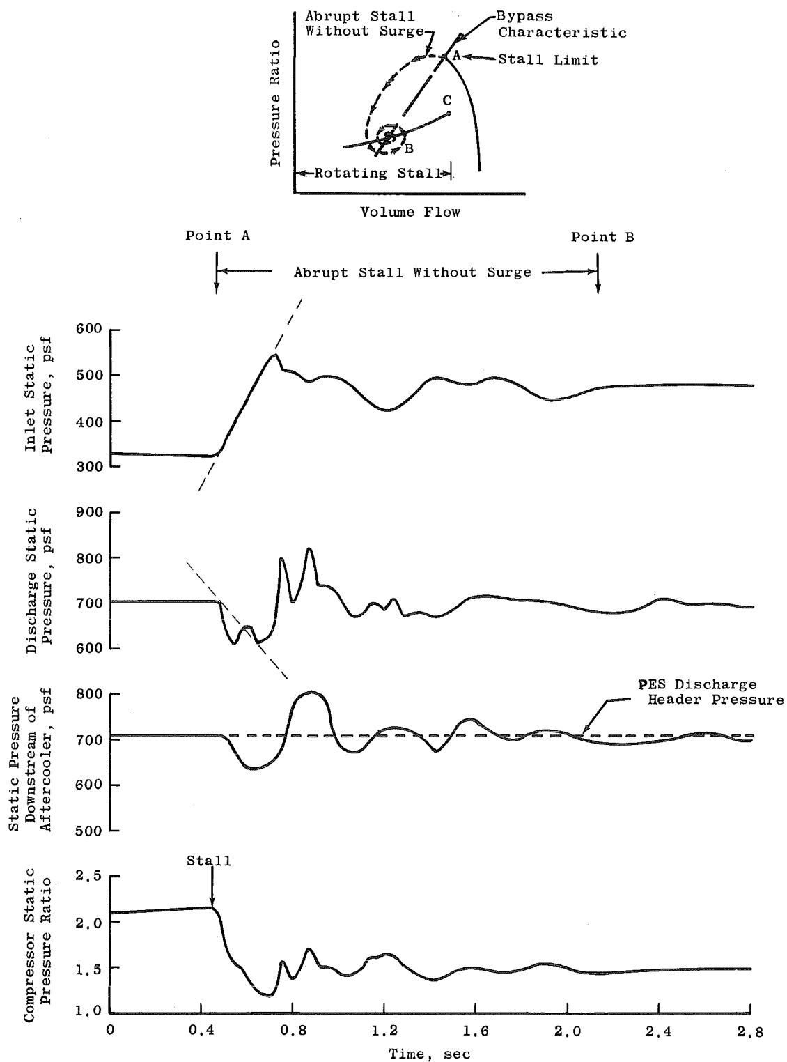
Fig. 14 Transient Compressor Measurements - Compressor Stall
