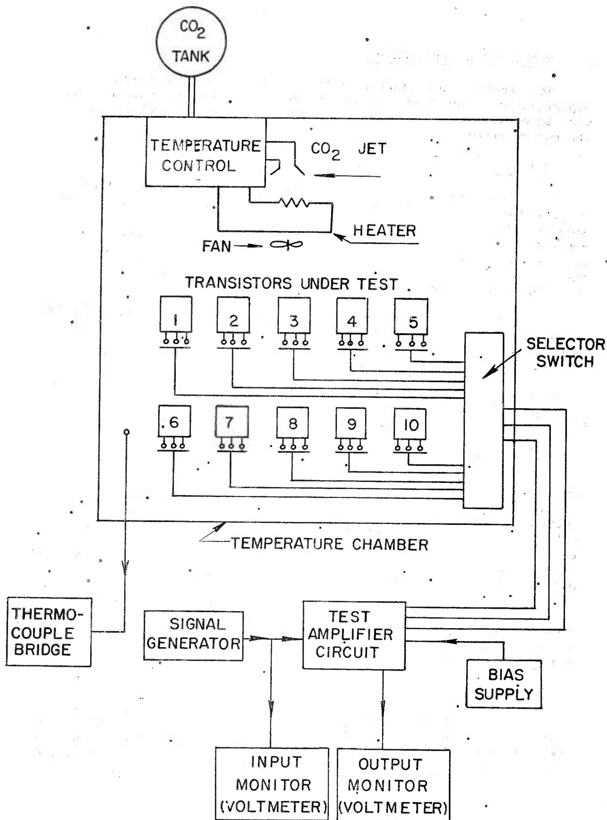
Figure 5. Environmental and monitoring systems.
