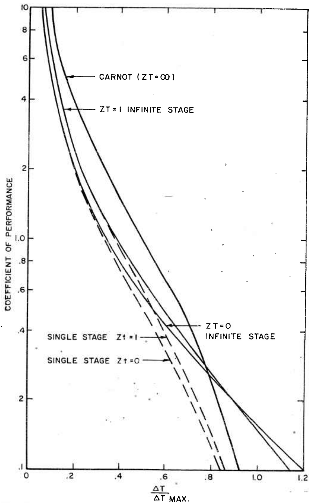
Figure 10. The maximum value of the coefficient of performance that can be obtained with single- and infinite-stage refrigerator shown as a function of the parameter \Delta T/\Delta T_{\text{max}} .
