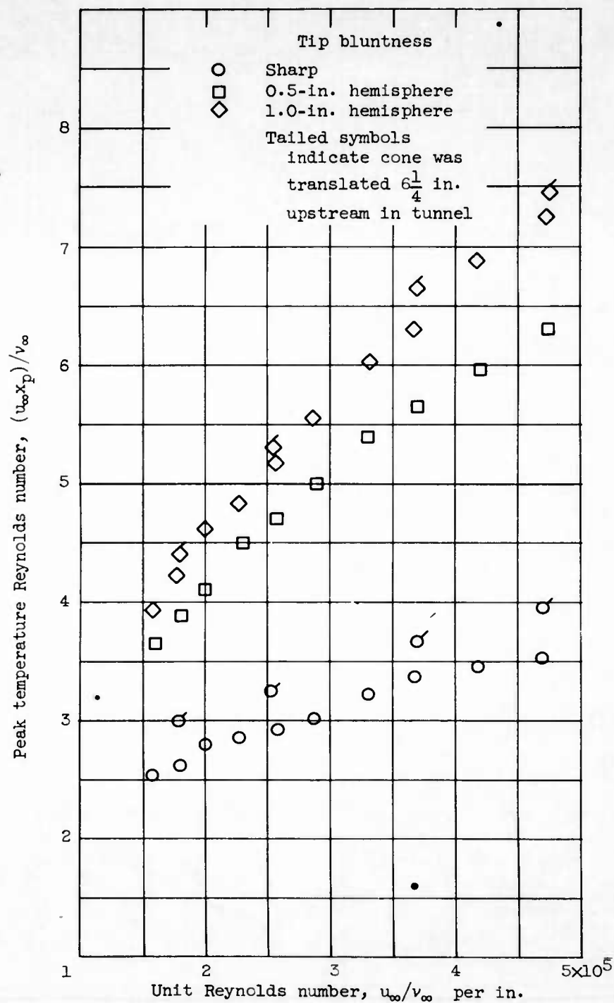
Figure 9. - Equilibrium peak temperature location on cone as function of unit Reynolds number and tip bluntness.
