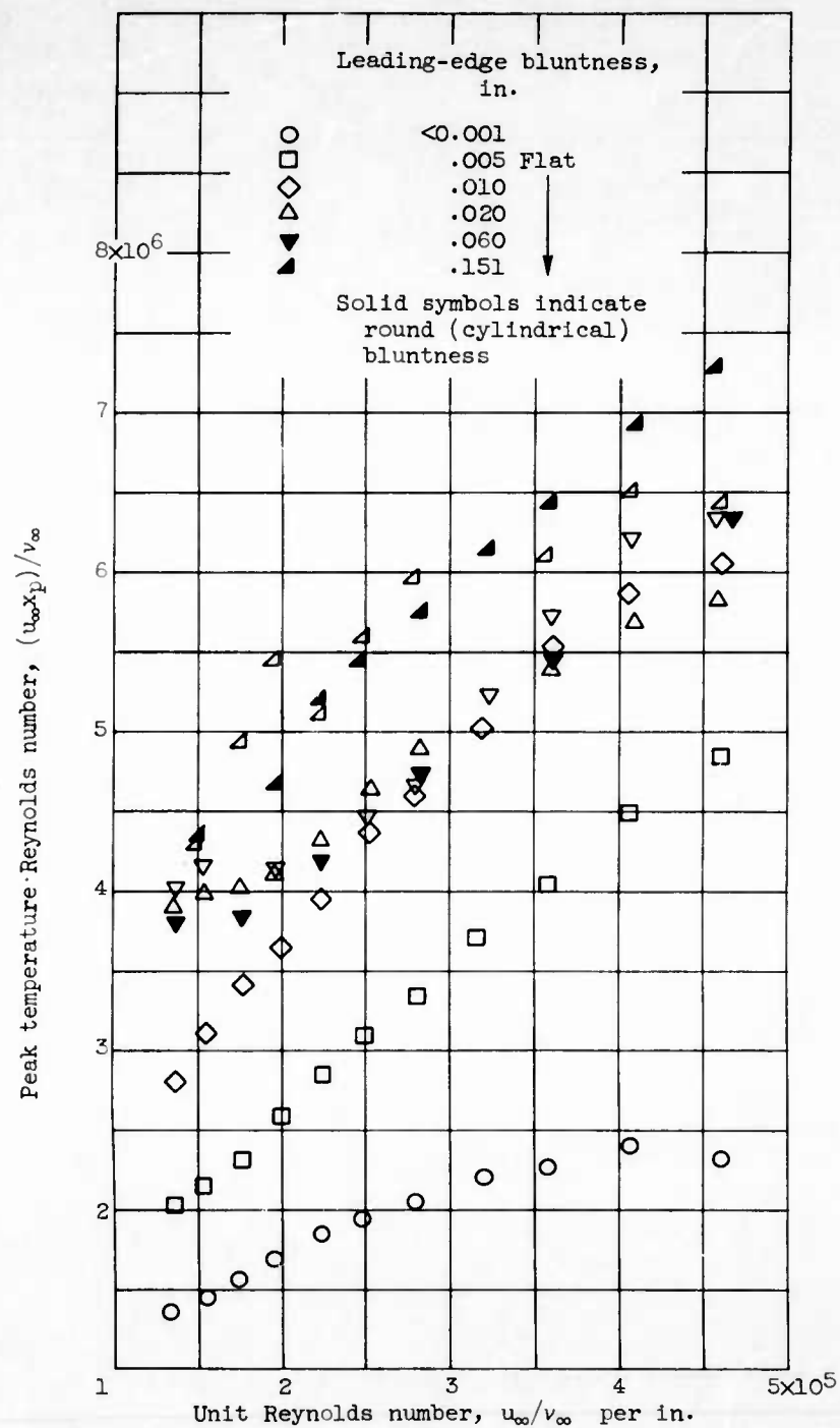
Figure 7. - Equilibrium peak temperature location on cylinder as function of unit Reynolds number and leading-edge bluntness.
