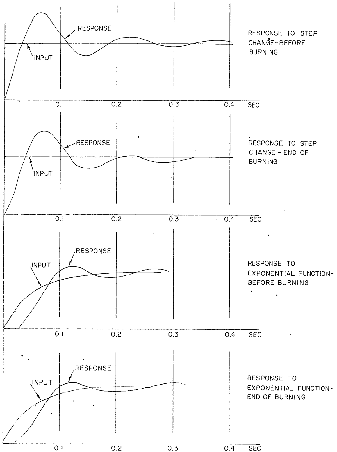
Fig. 21. Transient Response of Control System.
