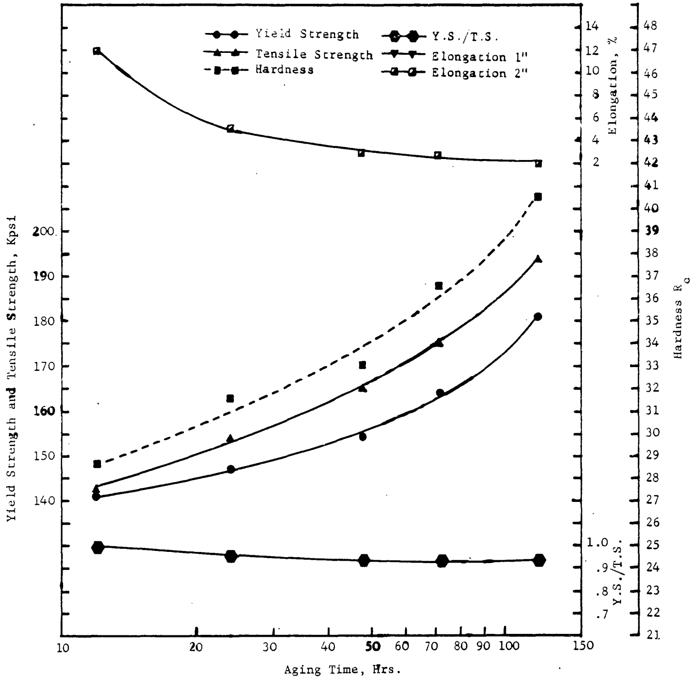
Fig. 10 Heat Treating Survey; B120VCA; Primary Direction
