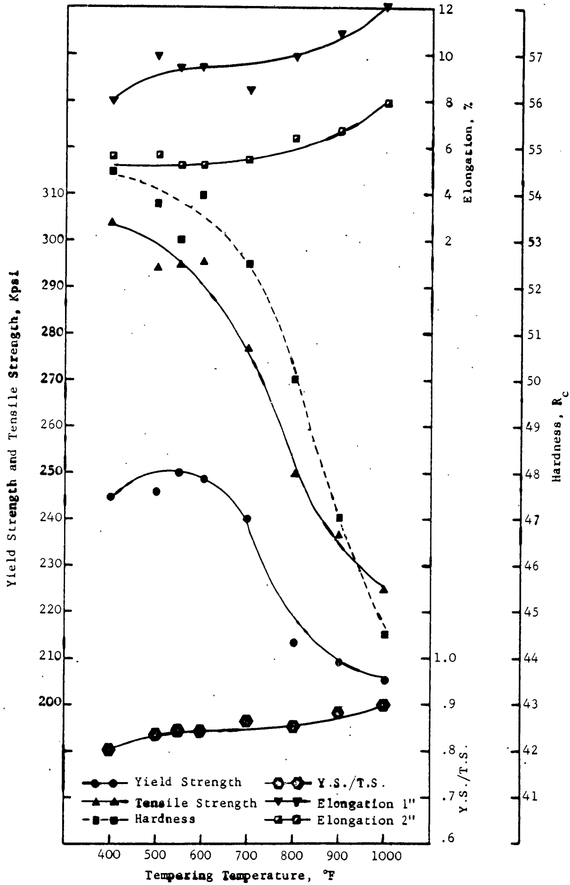
Fig. 6 Heat Treating Survey; 300M; Primary Direction
