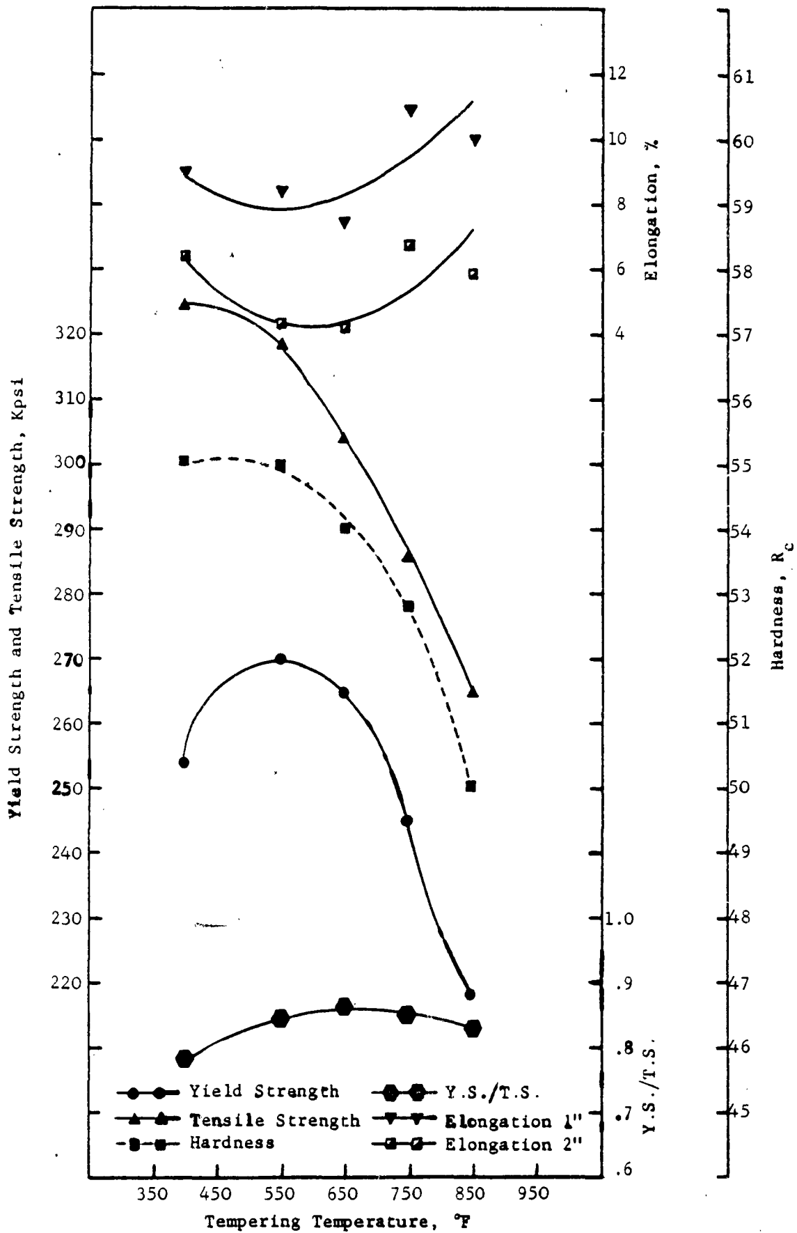
Fig. 12 Heat Treating Survey; R270; Primary Direction
