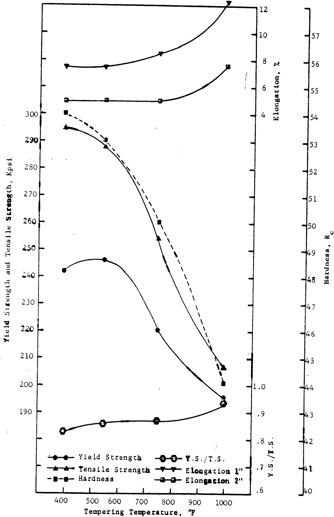
Fig. 11 Heat Treating Survey, 4137 Co; Primary Direction
