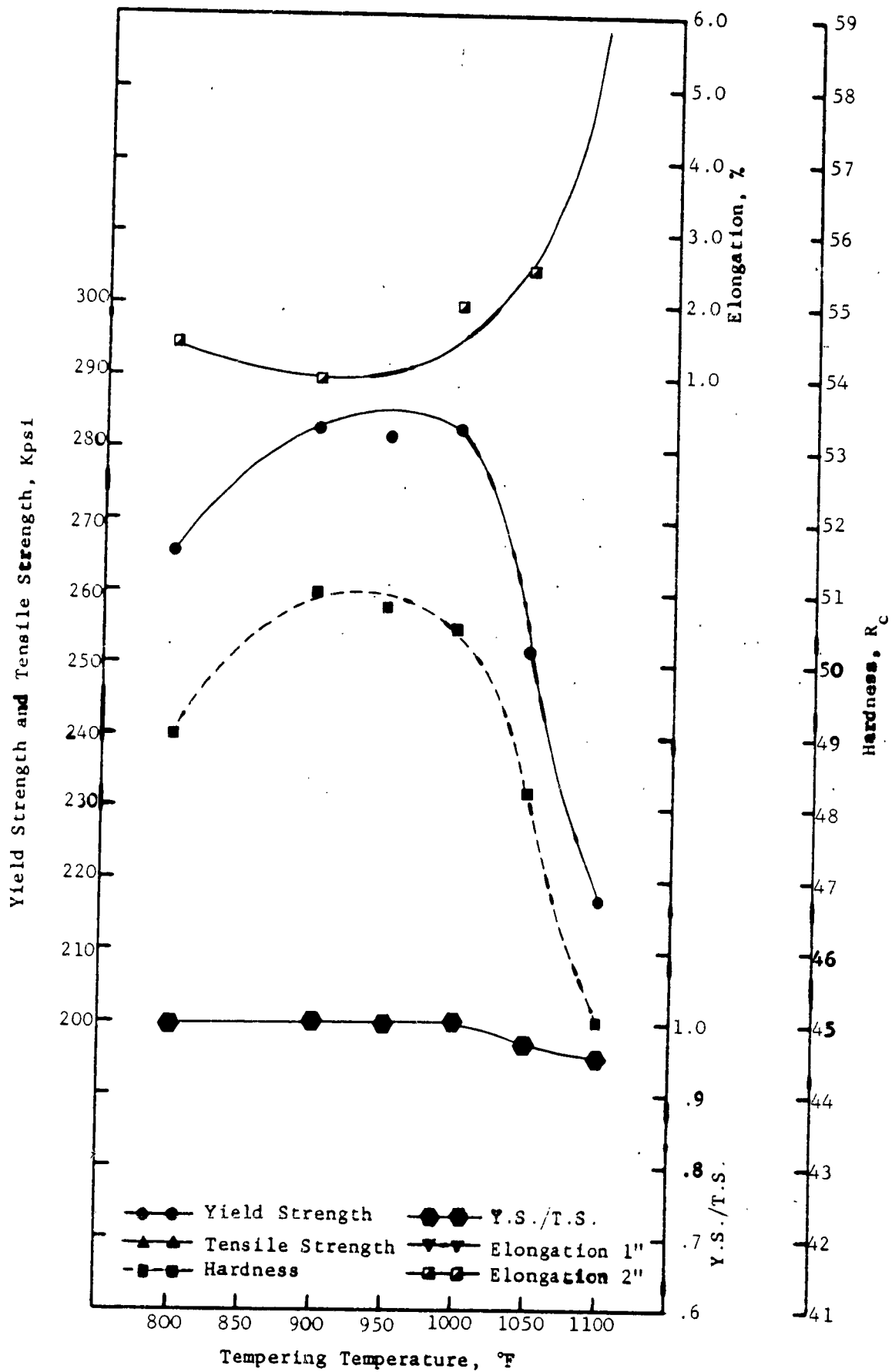
Fig. 8B Heat Treating Survey; PH15-7 Mo; Secondary Direction Note: Tensile Curve Not Shown; Closely Duplicates Y.S. Curve
