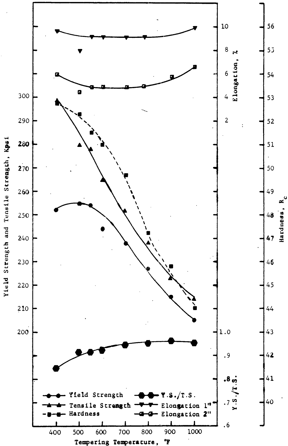
Fig. 5 Heat Treating Survey; D6Ac; Primary Direction
