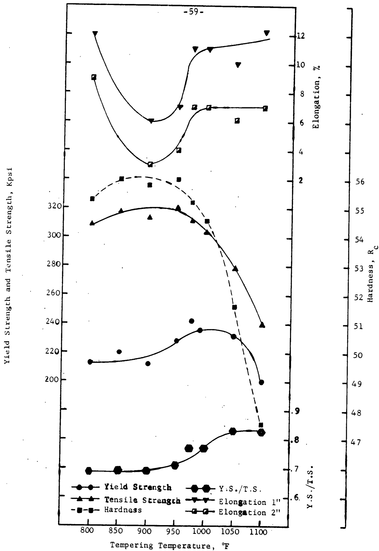
Fig. 7 Vascojet Heat Treatment Survey
