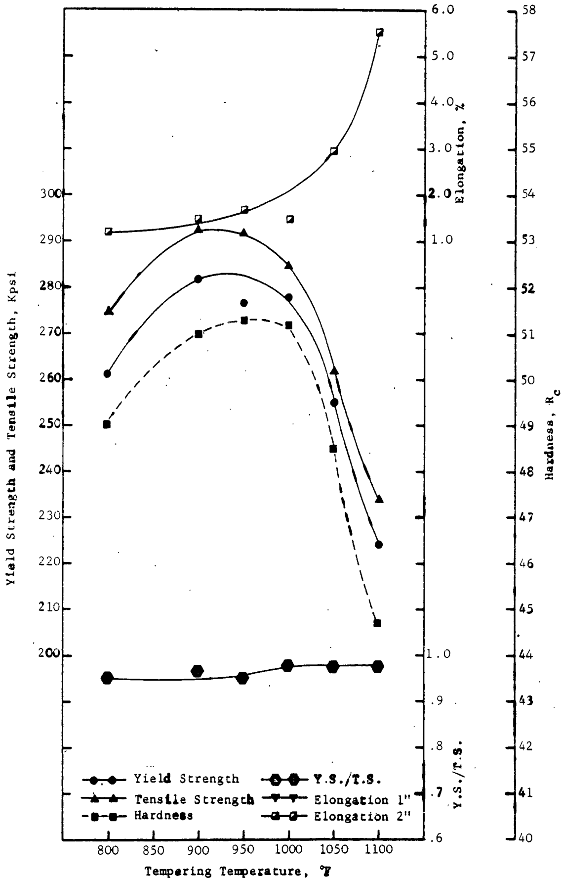
Fig. 8A Heat Treating Survey; PH15-7 Mo; Primary Direction
