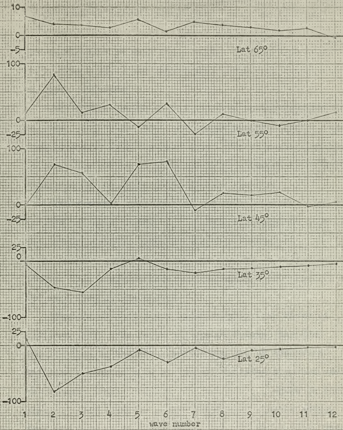
Figure 2. 33-day mean kinetic energy spectra by latitude belt for the period 31 December 1947 through 1 February 1948. Ordinate values are for the central latitude of each belt shown. Units are (m^2/sec^3/mb) \times 10^{-8} per ten-degree latitude belt.
