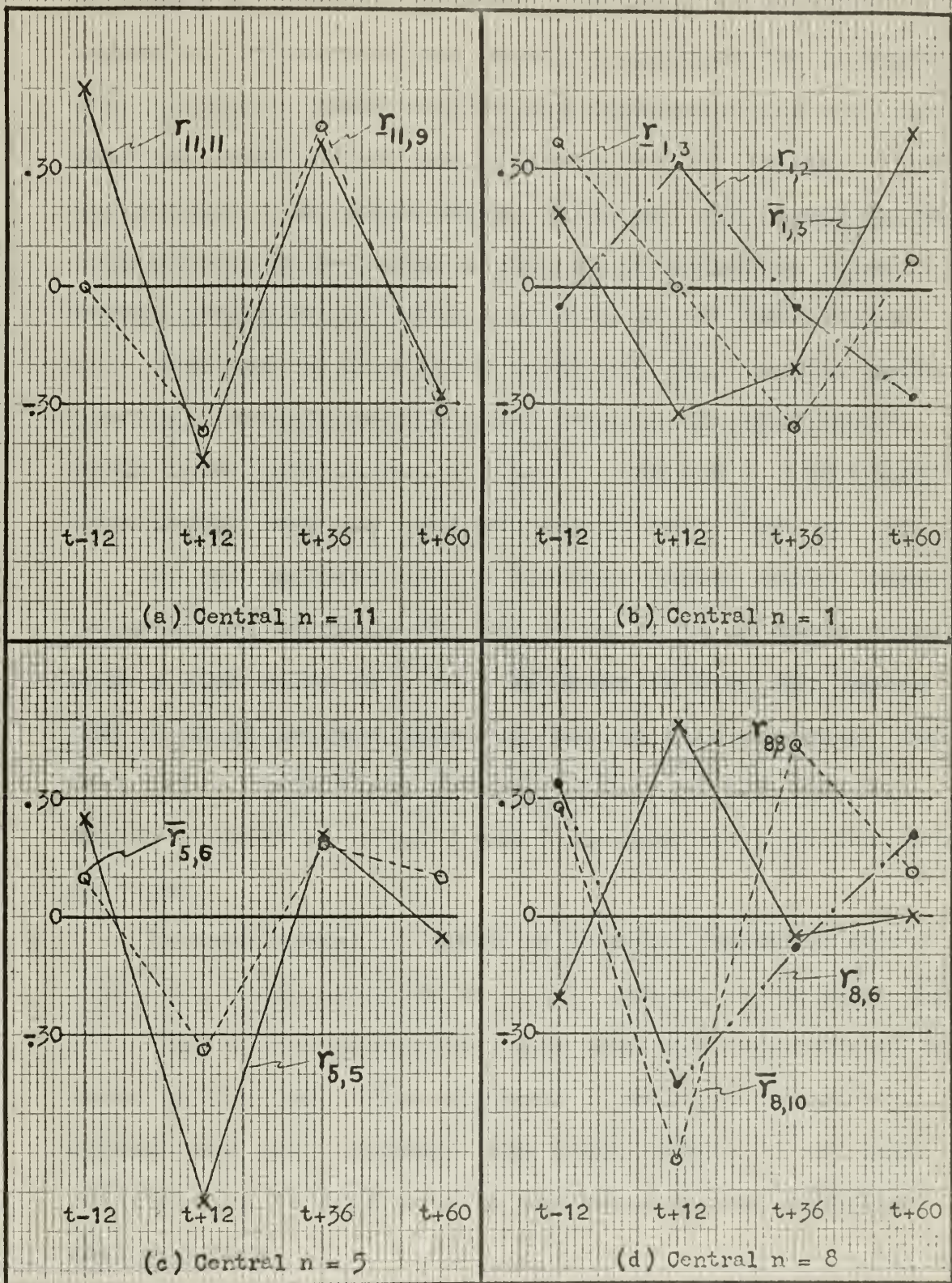
Figure 4. Sequential correlation coefficient sets of T^*(n) with \Delta KE for selected central n -values. Times are in hours from the computation time t of T^*(n) . Values of |r| > 0.30 are significant at the 90% level of belief.
