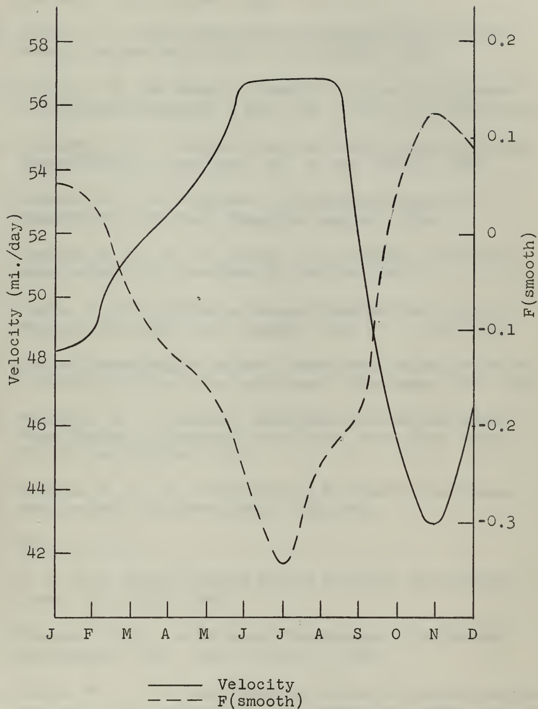
PLATE 7. Mean annual variation of F(smooth) compared with the mean annual variation of Gulf-Stream velocities Florida-South Carolina area
