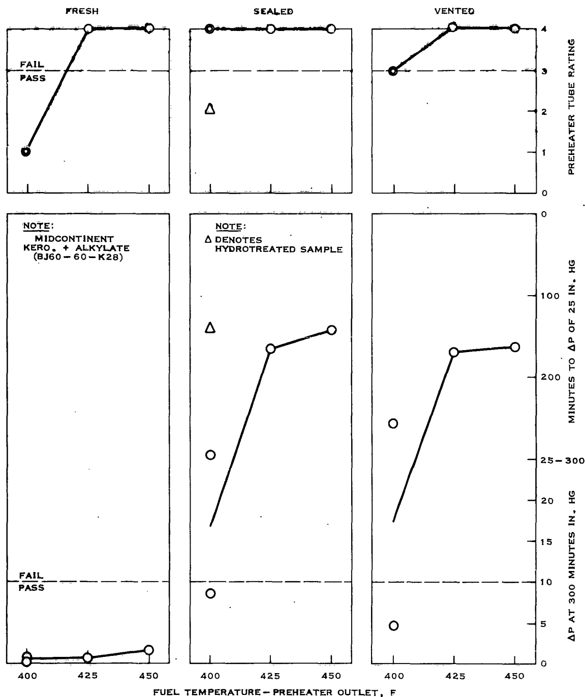
FIGURE 36 EFFECTS OF 26 WEEKS STORAGE AT 110F ON CFR FUEL COKER RATINGS AT VARIOUS TEMPERATURES FOR A JP-6 JET FUEL
