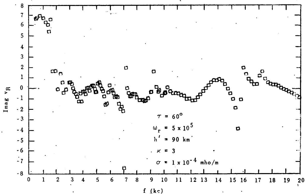
FIG. 3.25. REAL AND IMAGINARY PARTS OF CROSSED-LOOP VOLTAGE RATIO VS FREQUENCY FOR SUMMER-NIGHT MODEL IONOSPHERE, POOR GROUND, D = 2000 km, \phi_s = 0 .
