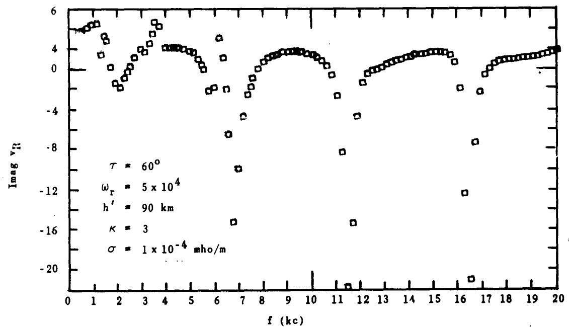
FIG. 3.29. REAL AND IMAGINARY PARTS OF CROSSED-LOOP VOLTAGE RATIO VS FREQUENCY, FOR SUMMER-NIGHT MODEL IONOSPHERE EXCEPT \omega_r = 5 \times 10^4 , POOR GROUND, D = 500 \text{ km} , AND \phi_g = 0 .
