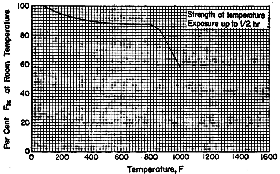
Figure 2.2.4.2.1(a). Effect of temperature on the ultimate tensile strength ( F_{tu} ) of AM-350 stainless steel (SCT).
