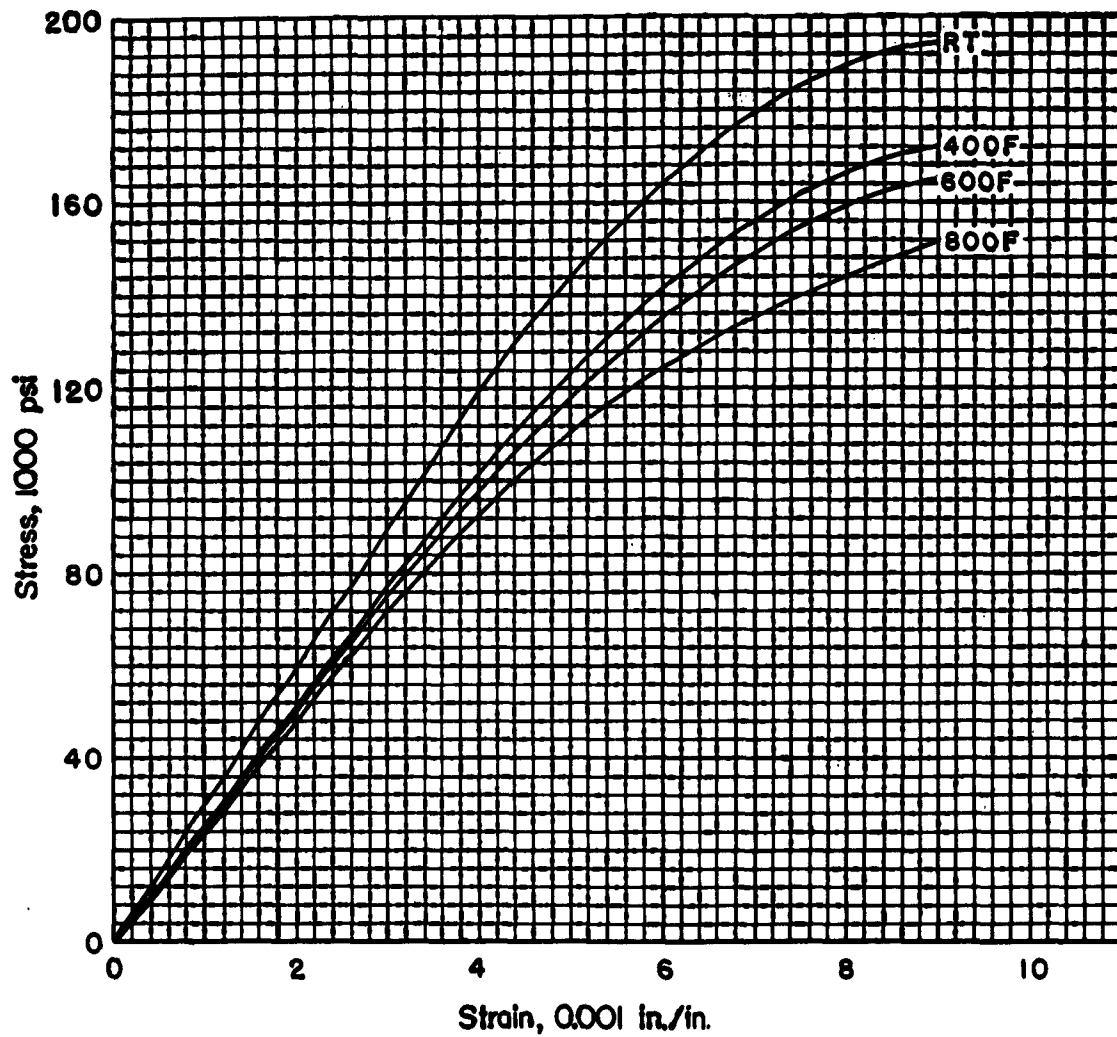
Figure 2.2.4.2.6(b). Typical compressive stress-strain curves for AM-350 stainless steel (SCT) at room and elevated temperatures.
