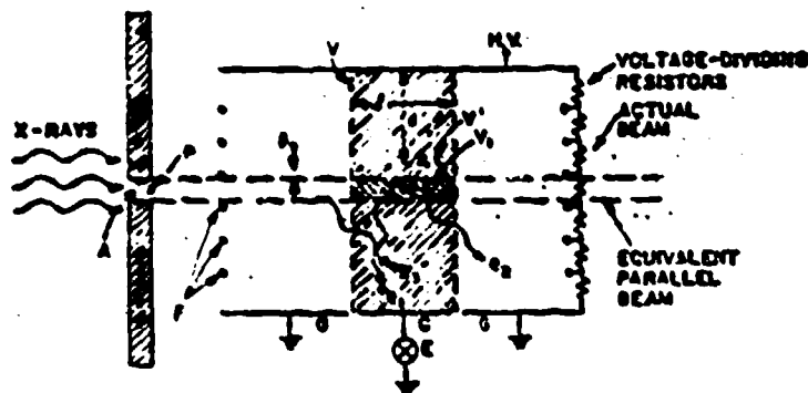
Fig. 5 - The conventional guarded-field, parallel-plate, free-air ionization chamber. Ionization is collected from the volume v .
