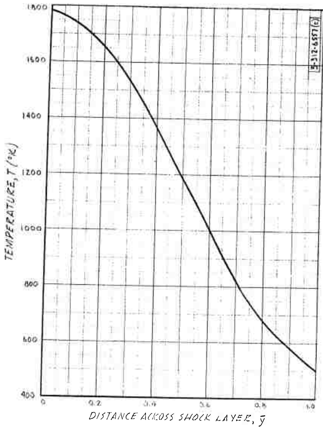
Fig. II-12(c). Temperature distribution across shock layer. x/r_n = 23 . Altitude 150,000 feet.
