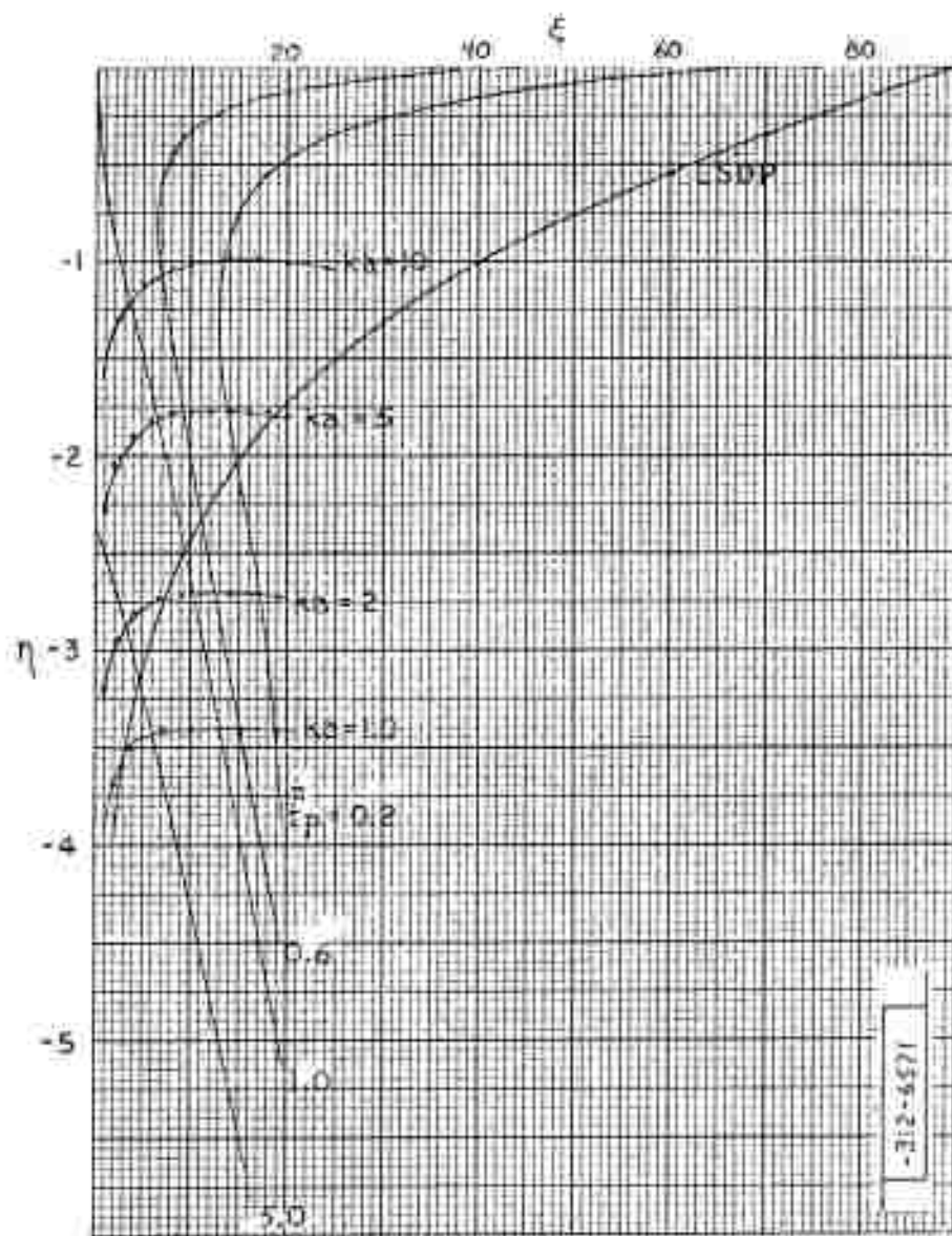
Fig. IV-11. Root loci of TE_{0-5} mode.
