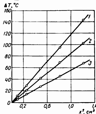
Fig.2. Temperature distribution near the center of the short tungsten sample; 1-temperature at center 1600 ; 2- 1400 ; 3-1600 C.
