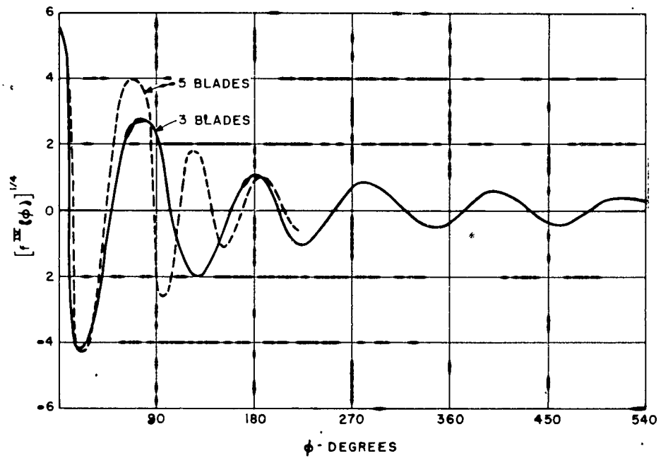
FIG. 2.2 PLOT OF [r^{1/2} \xi(\phi)]^{1/4} FOR AXIAL INDUCED VELOCITY FOR \nu=2 \beta_{t0}=20^\circ
