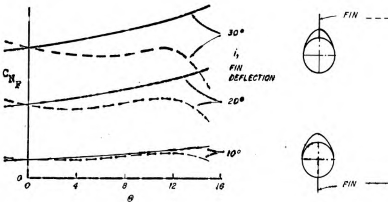
Figure 2 - Individual Fin Loads - Top and Bottom
