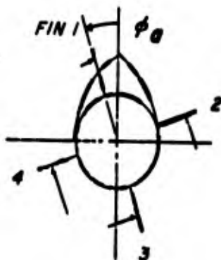
Figure 8 - Fin Forces with \theta_a = 0^\circ
