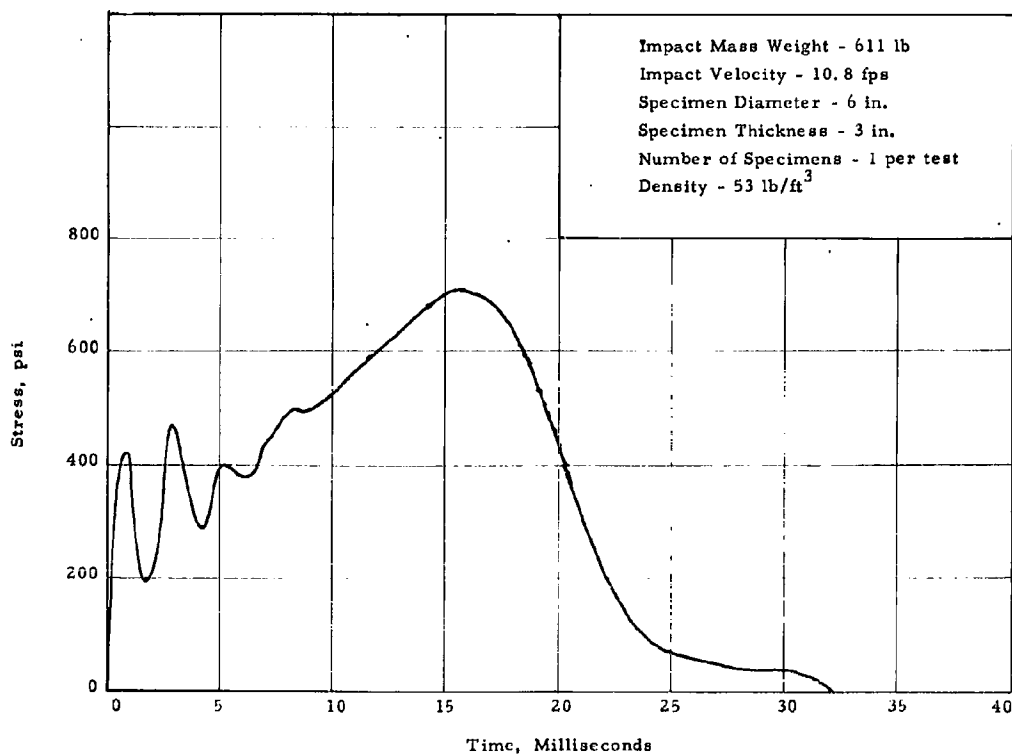
Fig. 10. Dynamic Stress vs Time Curve at 10.8 fps.
