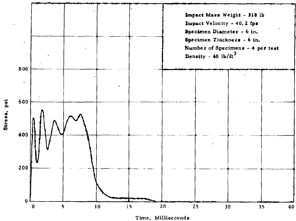
Fig. 18. Dynamic Stress vs Time Curve at 40.2 fps.
