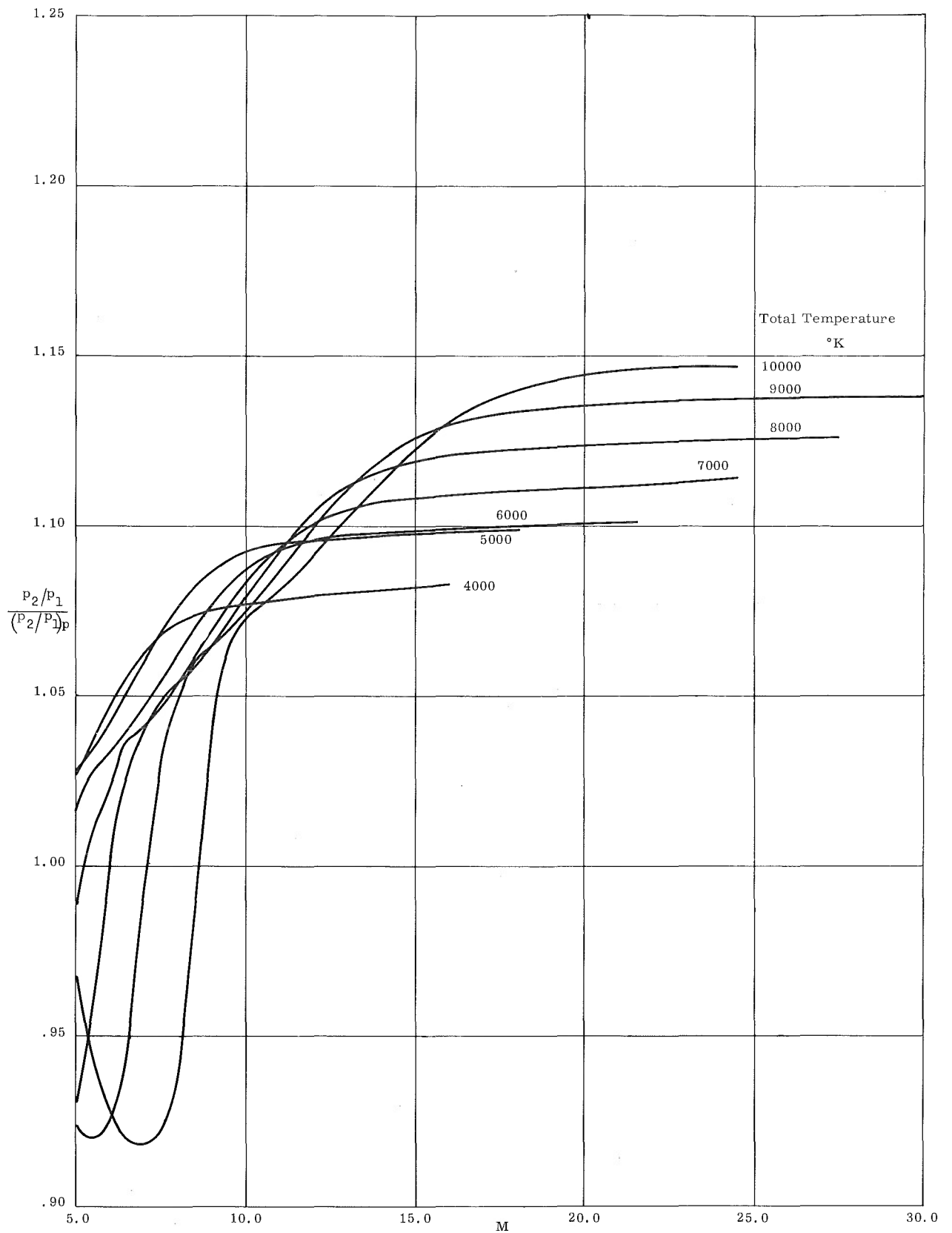
h. p_2/p_1 Fig. 2 -- Continued
