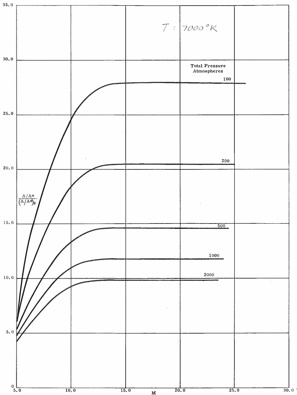
e. A/A^* Fig. 3 -- Continued
