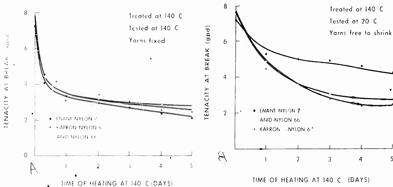
a. Yarns fixed b. Yarns free to shrink Figure 3. Strength loss in Enant, kapron, and anid exposed to 140°C (source: Russian article, Ref. 25)
