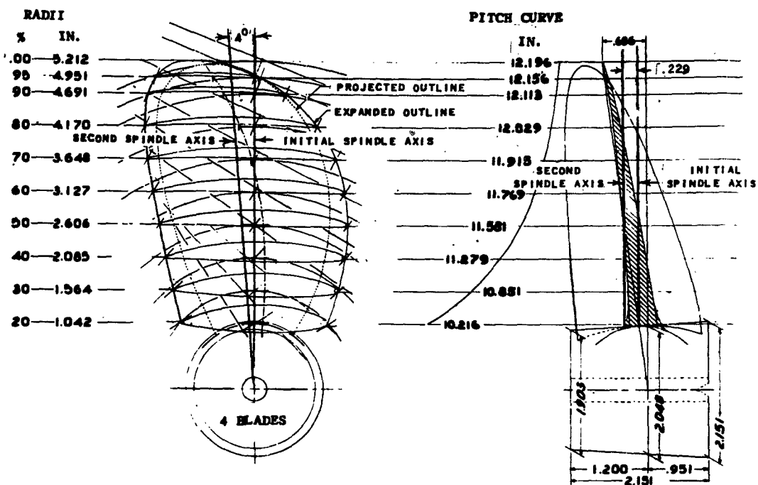
Figure 7 - Drawing of Example Propeller
