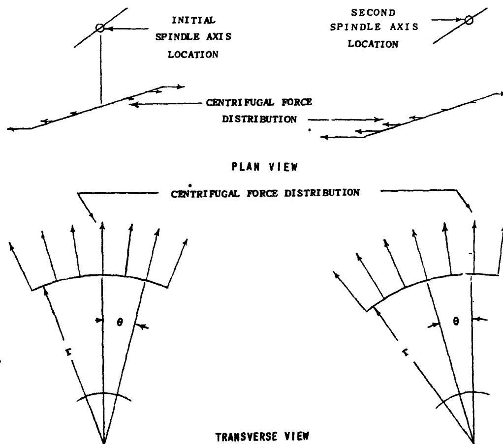
Figure 6 - Effect of Changed Spindle Axis Location on Centrifugal Blade Spindle Torque
