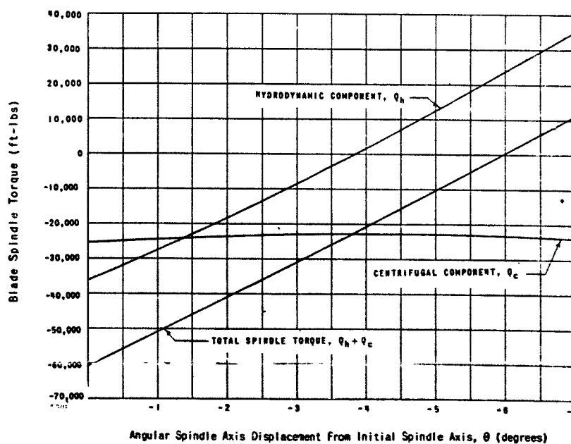
Figure 10 - Variation of Spindle Torque with Location of Spindle Axis for Example Propeller
