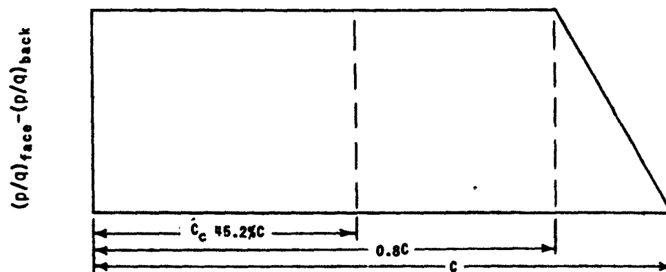
Figure 8 - Lift Distribution of a=0.8 Mean Line
