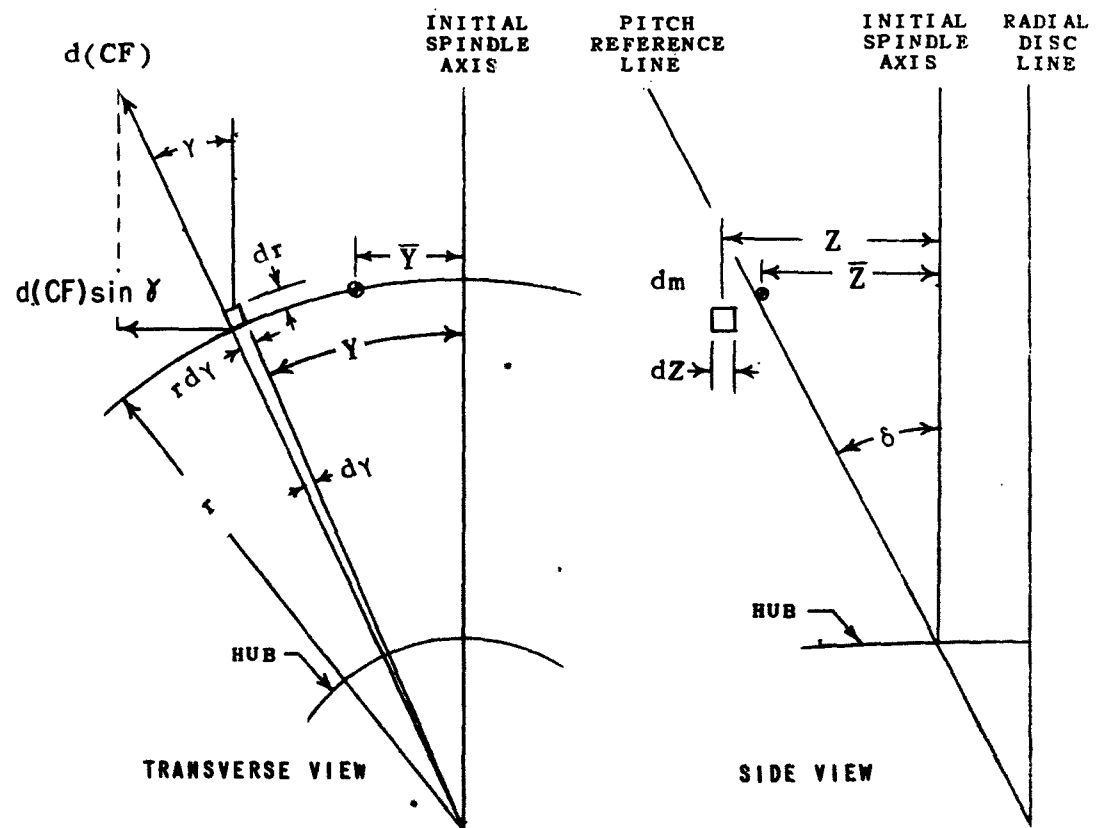
Figure 4 - Diagram of Centrifugal Forces and Distances to Initial Spindle Axis
