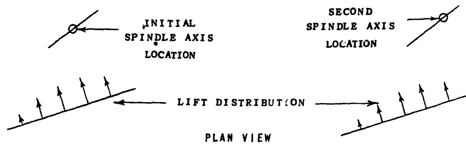
Figure 5 - Effect of Changed Spindle Axis Location on Hydrodynamic Blade Spindle Torque
