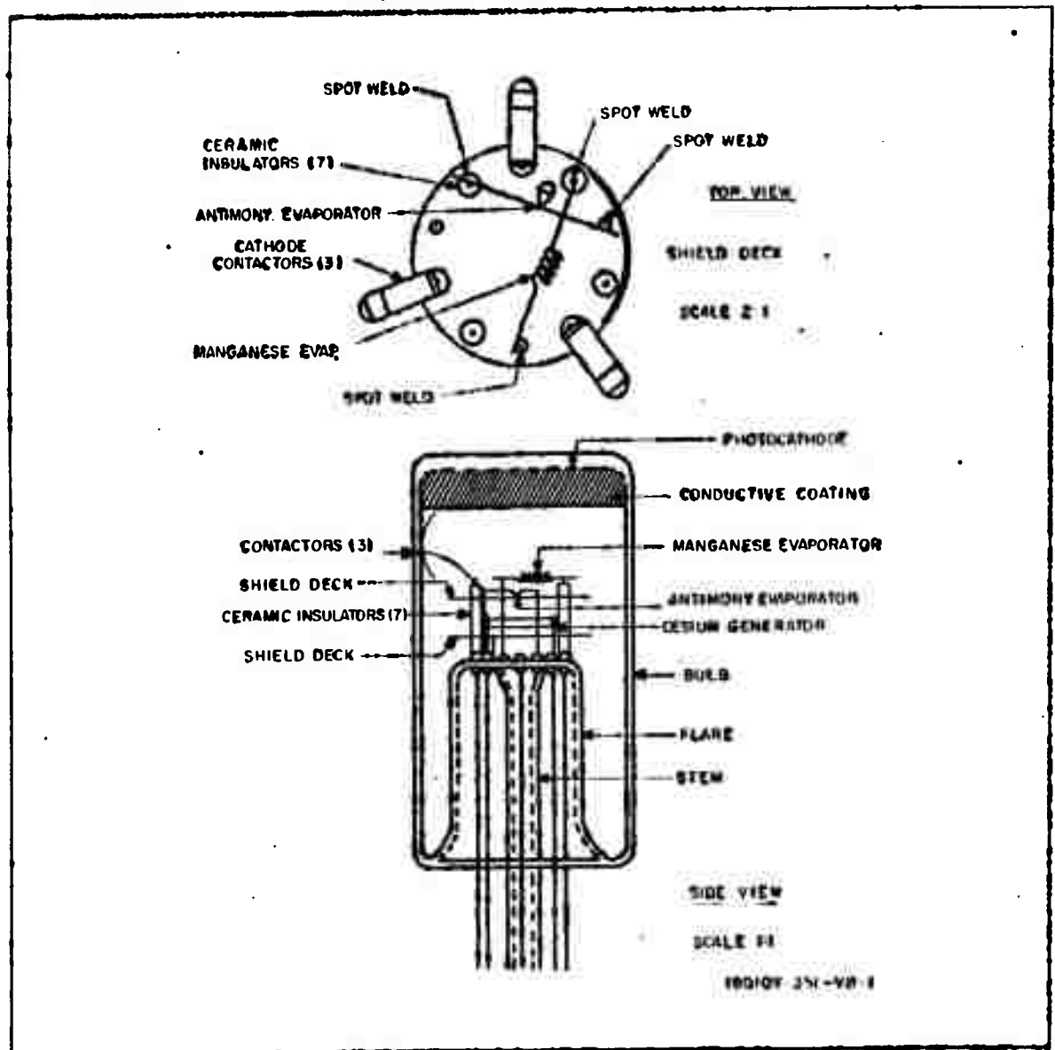
Figure 1. WX-4220 Photoemission Control Tube
