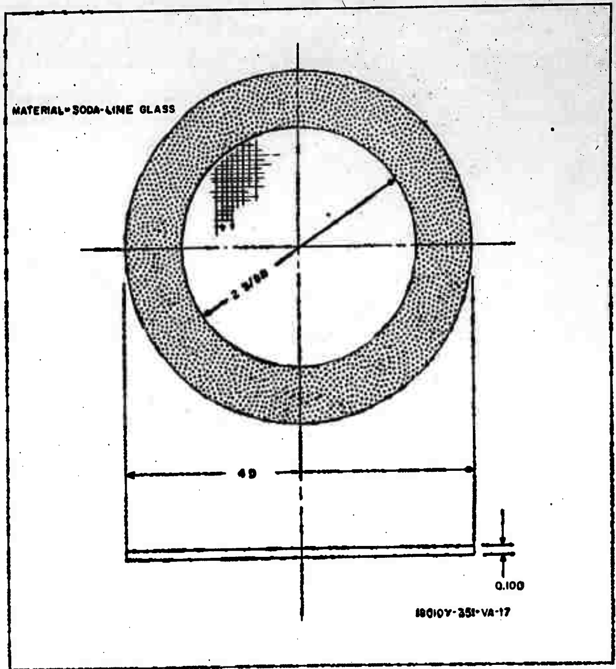
Figure C-4. WX-4209 Photoemissive Power Generator (A) Photocathode Substrate
