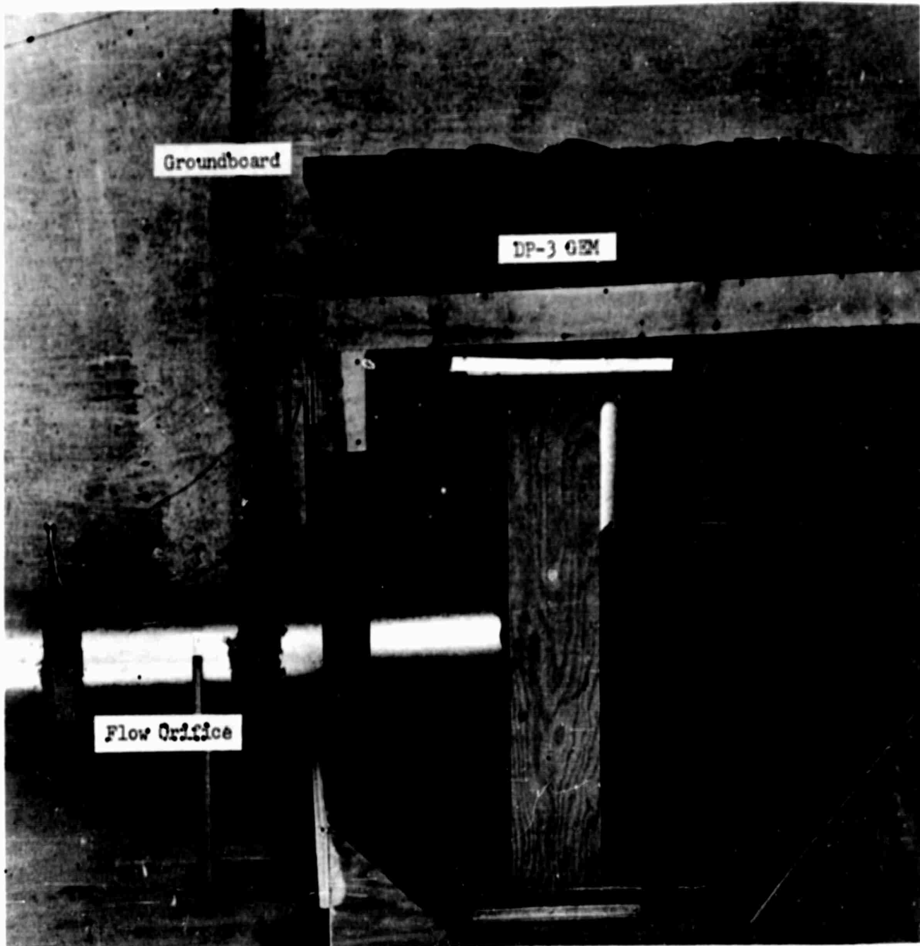
FIGURE 11: STATIC TEST DP-3 GEM-GROUND BOARD-MODEL ARRANGEMENT AND FLOW MEASUREMENT CRIFICE
