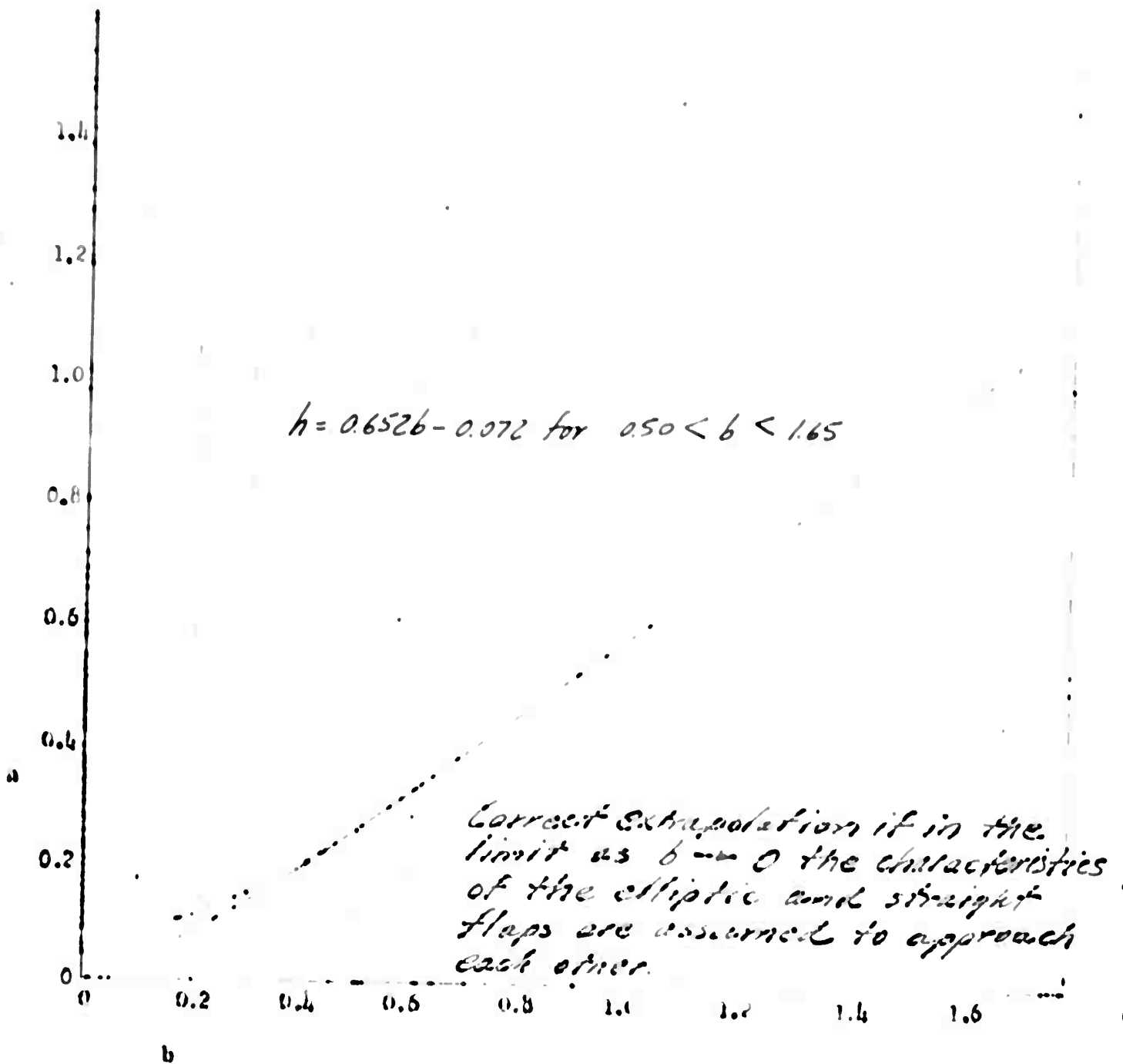
FIGURE 39: ELLIPTIC FLAP: h = f(b) FOR MAXIMUM RATE OF CHANGE OF \frac{I}{q_a^2} WITH h
