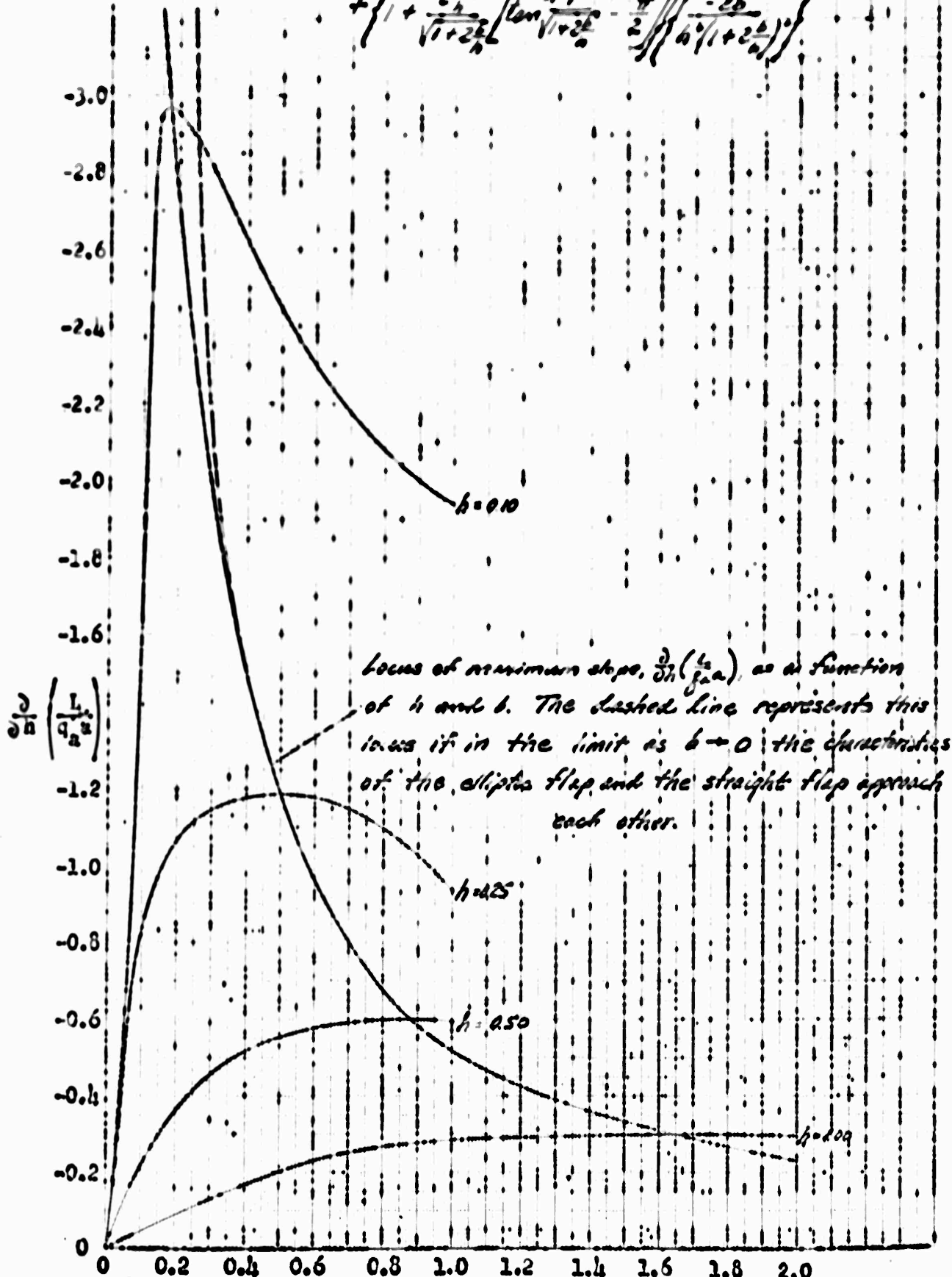
FIGURE 38: RATE OF CHANGE OF \frac{L}{q_2 a} WITH h FOR ELLIPTIC FLAP
