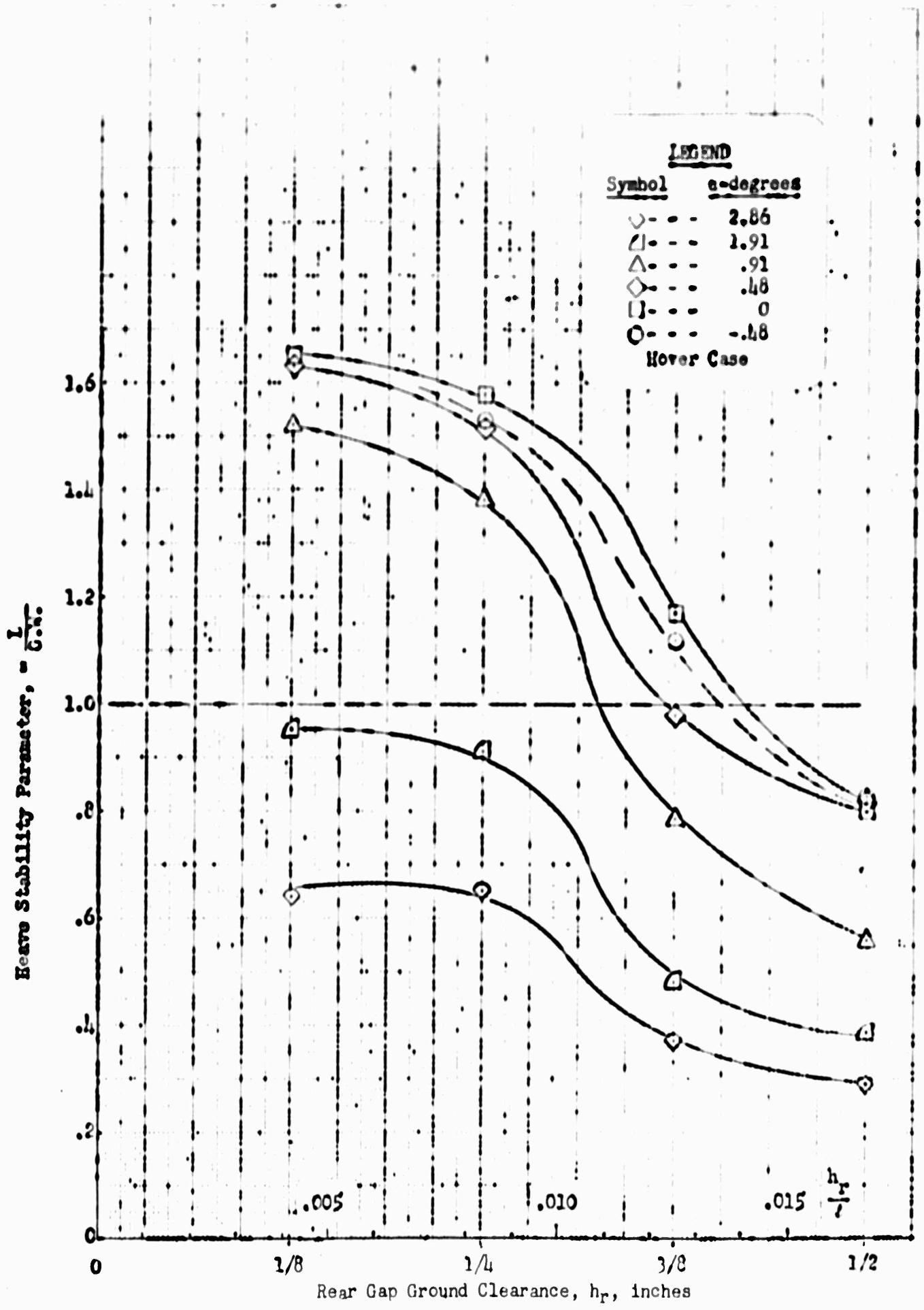
FIGURE 31: HEAVE STABILITY CHARACTERISTICS DP-3 GEM
