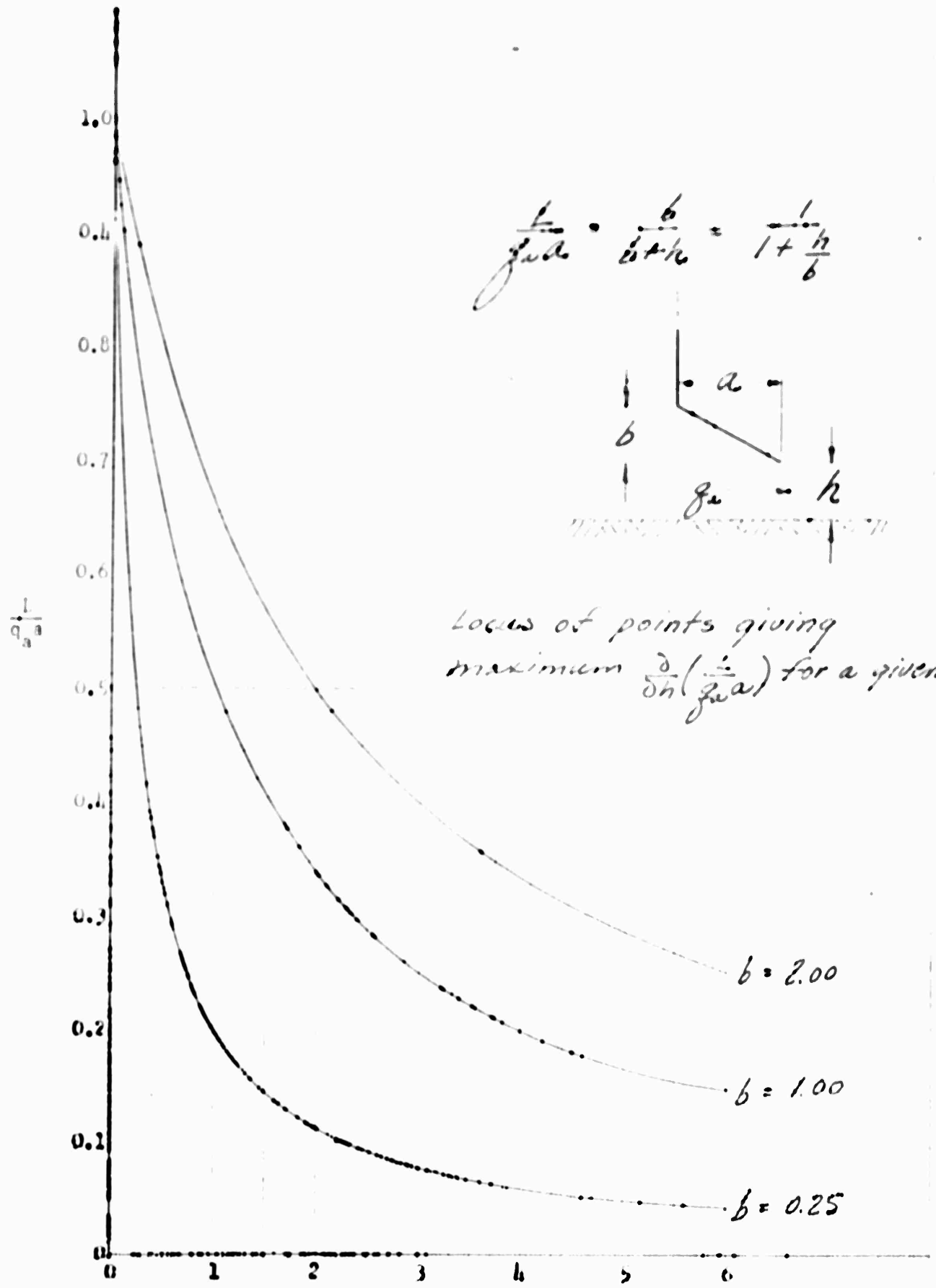
FIGURE 34: STRAIGHT FLAP CHARACTERISTICS
