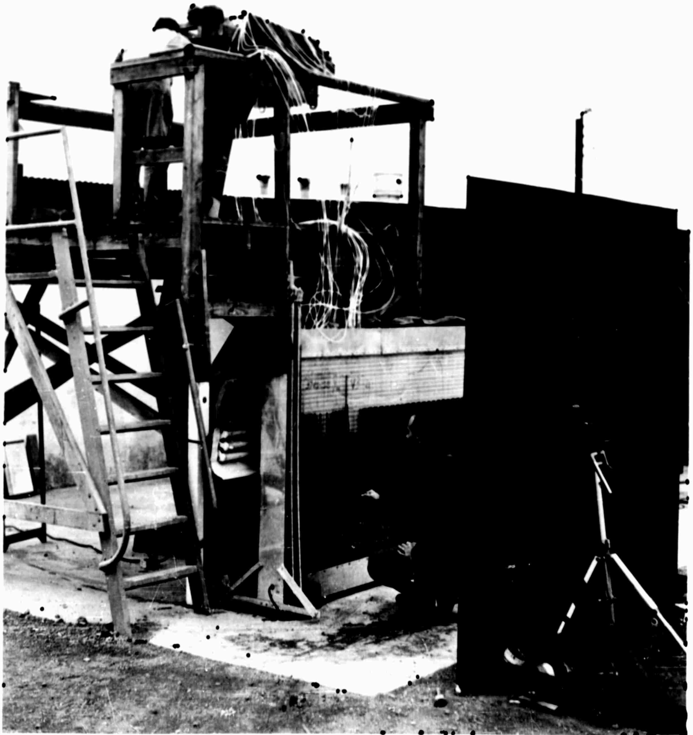
FIGURE 5: TWO-DIMENSIONAL DIFFUSER PLENUM MODEL TEST SET-UP
