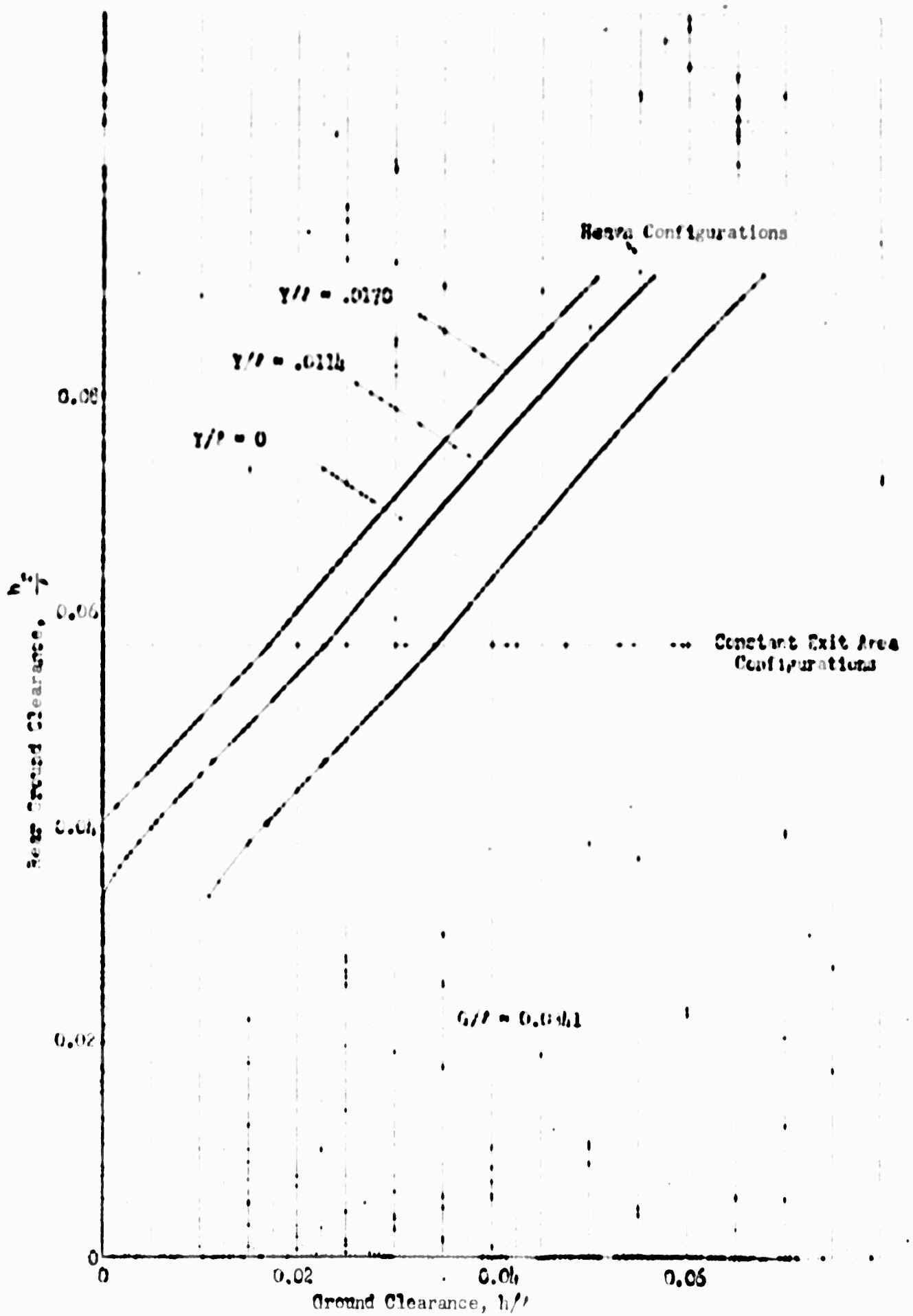
FIGURE 14: REAR GROUND CLEARANCE AS A FUNCTION OF FRONT GROUND CLEARANCE
