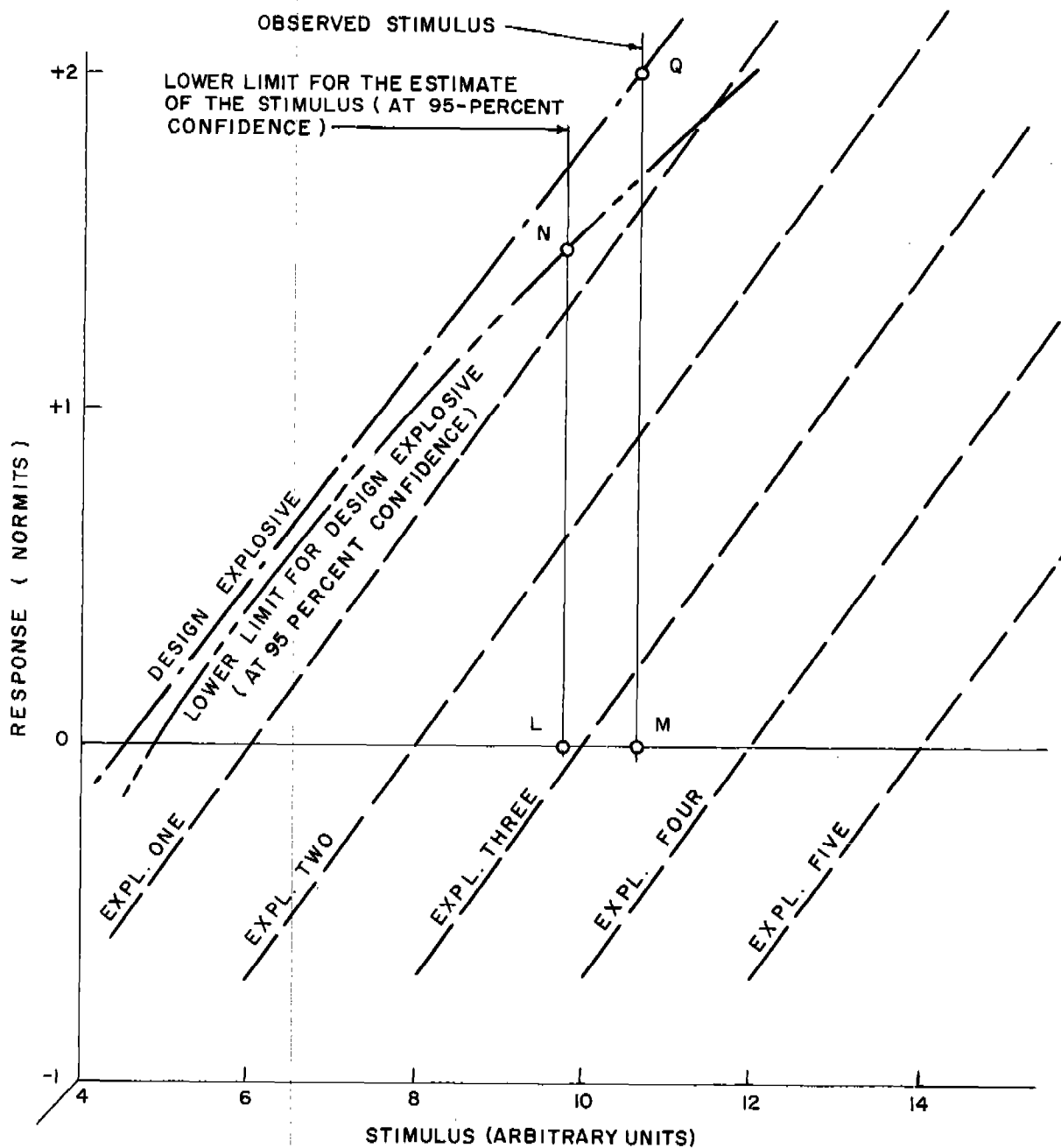
FIGURE 9.93 PREDICTION OF THE RELIABILITY OF AN EXPLOSIVE SYSTEM ON THE BASIS OF BRUCETON PLAN PERFORMANCE TESTS WITH VARICOMP EXPOSIVES
