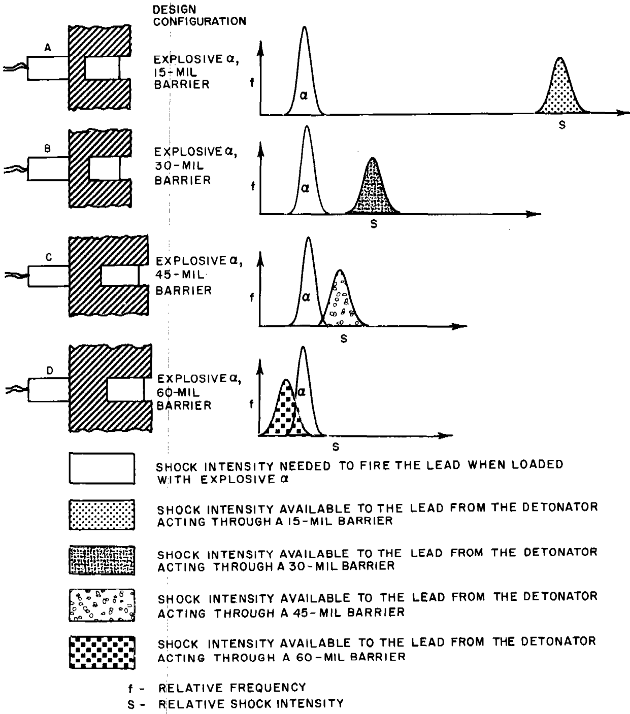
FIGURE 3.1 EXPLOSIVE PENALTY TESTING BY VARIATION OF BARRIER THICKNESS
