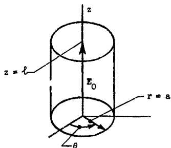
FIG. F.1--Coordinate system for cylindrical port of nonlinear dielectric.
