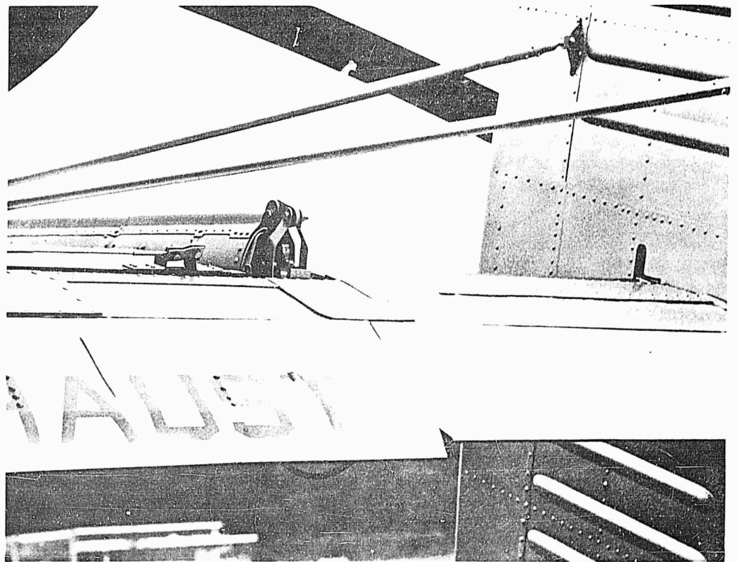
SPRING TAB POSITION WITH UP COLLECTIVE
