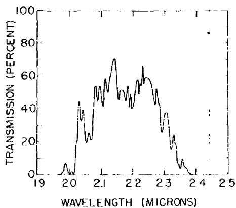
Fig. 9 - Atmospheric transmission for a 16.25-km path as a function of wavelength (from Ref. 6 (showing weak absorption structures in the 2\mu region)
