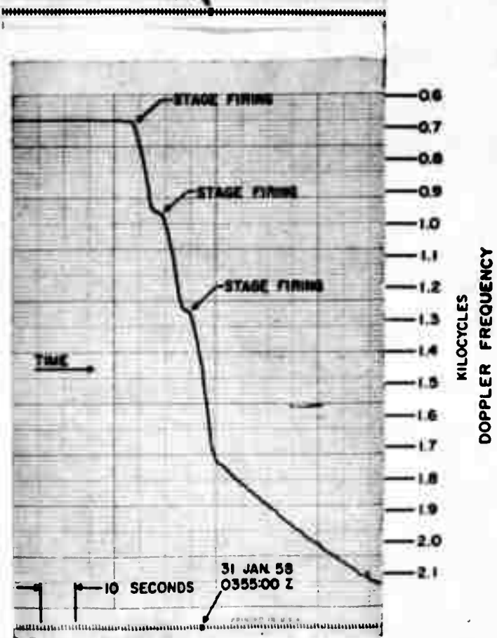
DOPPLER FREQUENCY RECORD OF THE LAUNCH OF EXPLORER I (58 ALPHA) TRACKED AT ABERDEEN PROVING GROUND, MD.
