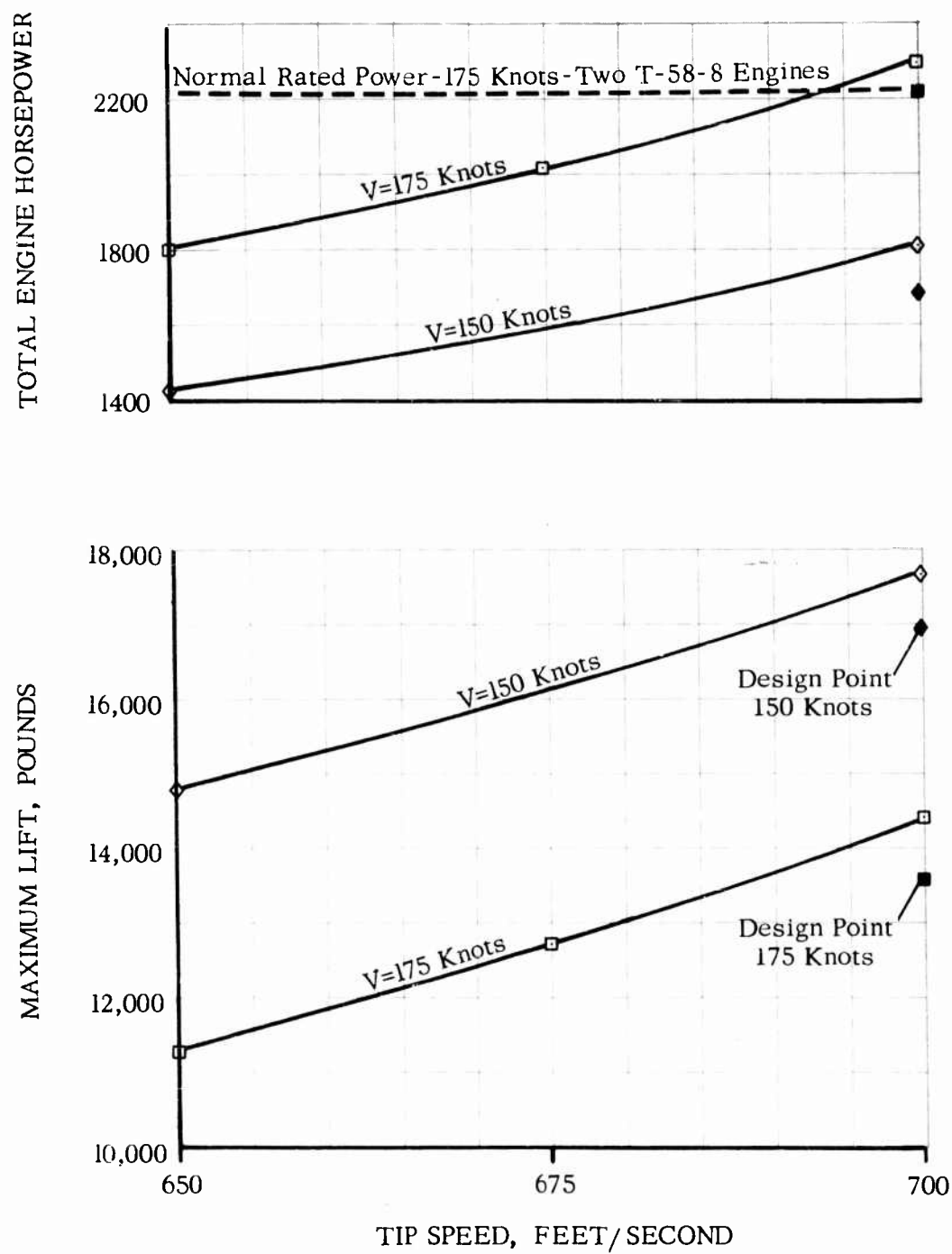
FIGURE 17. EFFECT OF TIP SPEED ON MAXIMUM LIFT CAPABILITY
