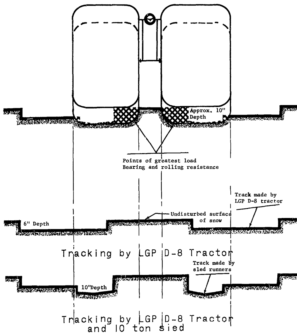
FIG. 29 TRACKING OF LGP TRACTER, D-8, 10 TON SLED AND RLT ON THE GREENLAND ICECAP. Scale: \frac{1}{2} "=1'-0"
