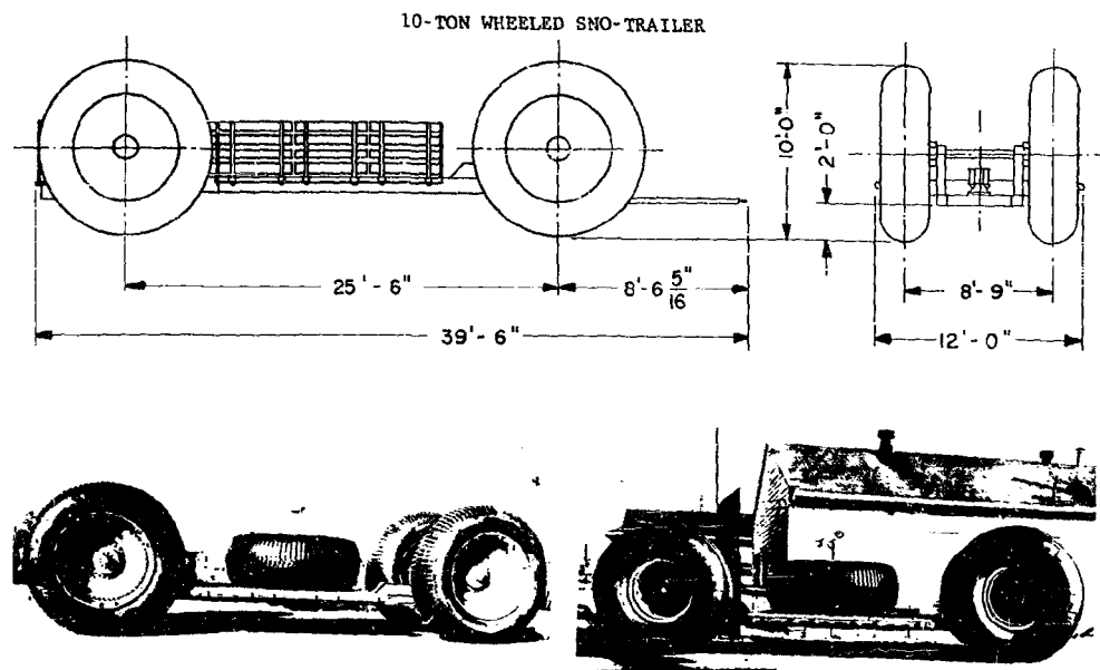
Sno-Trailer With Firestone Tires
