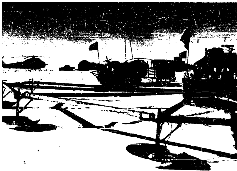
Figure 63: "W" System crevasse detector and Sperry Marine Radar mounted on pathfinder weasel.
