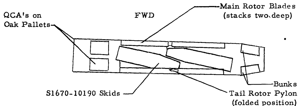
Floor Plan of C-124 Loaded with Two H-34C's
