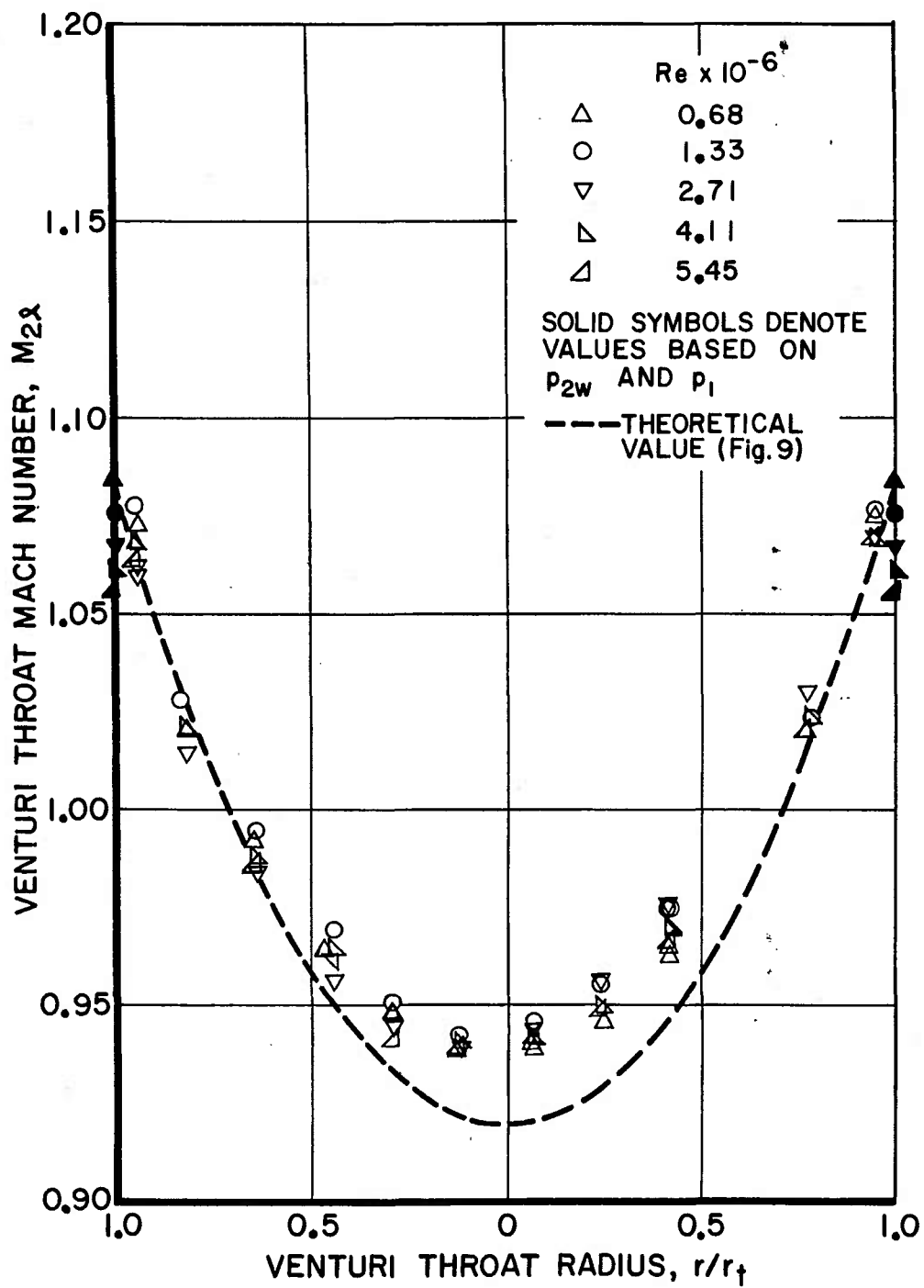
Fig. 23 Comparison of Theoretical and Experimental Mach Number and Weight-Velocity Profiles across Venturi Throat
