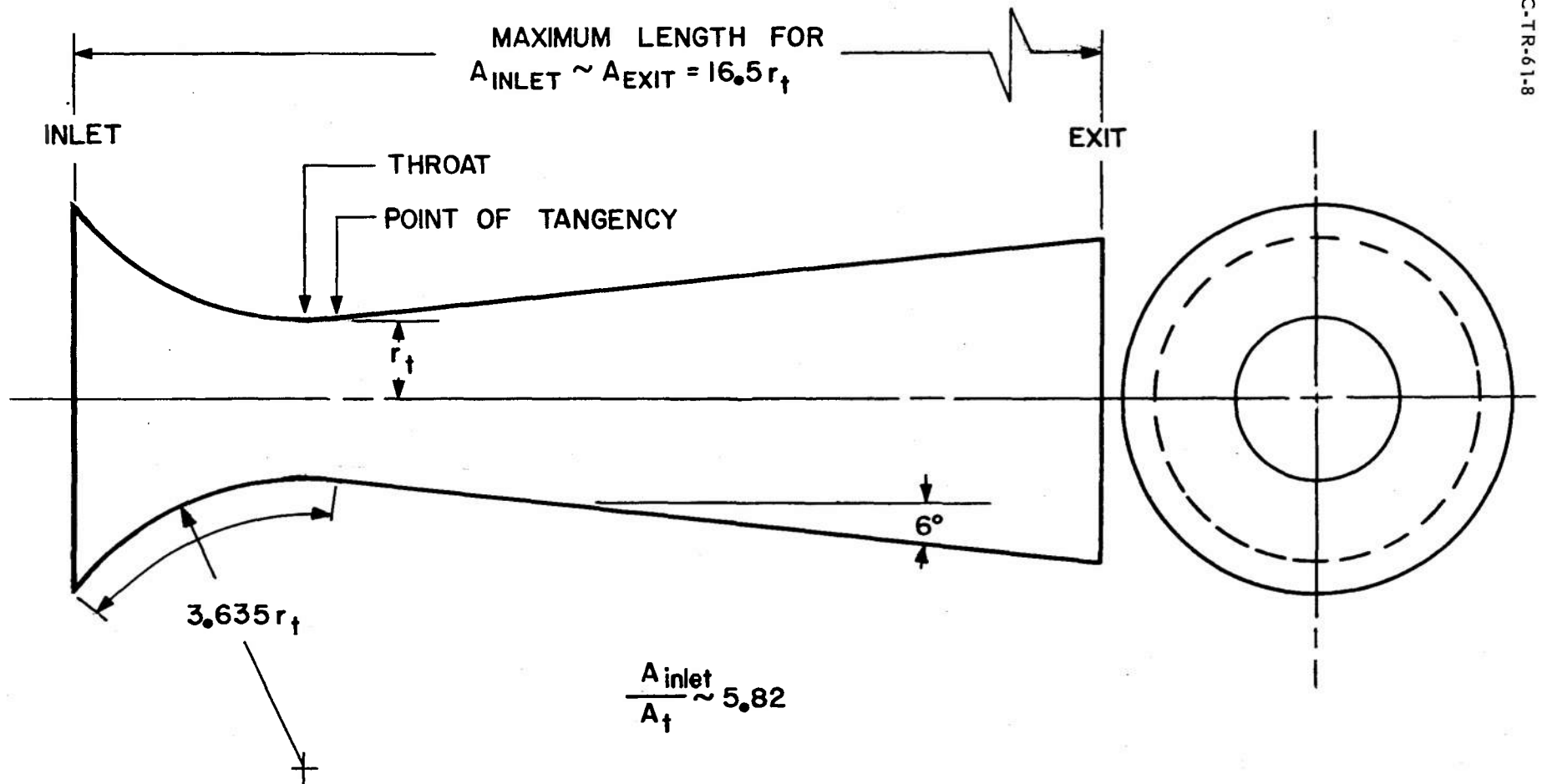
Fig. 4 Schematic of Venturi Design for Operation at Critical Flow Conditions
