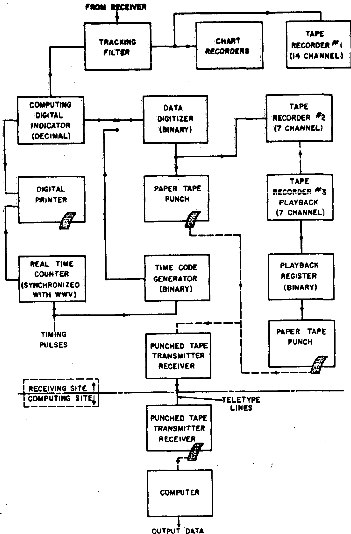
SIMPLIFIED BLOCK DIAGRAM — DOPLOC SYSTEM DATA HANDLING FIGURE 23
