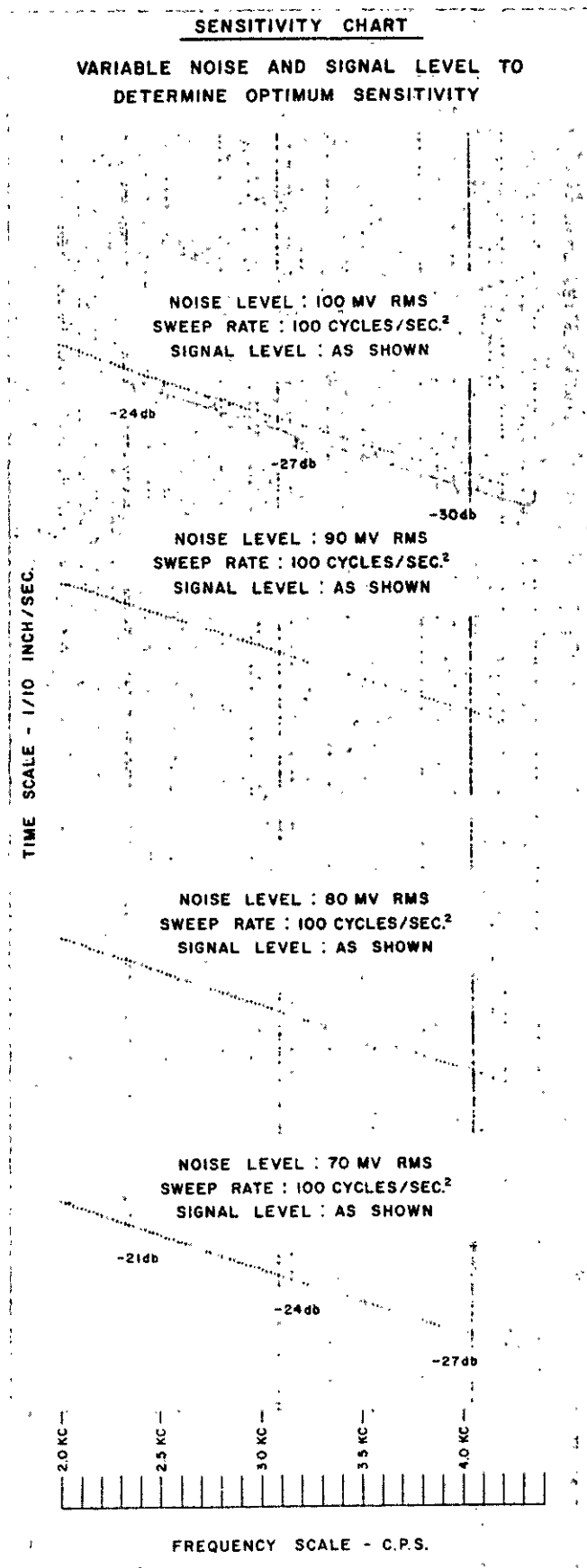
Figure 51 Sensitivity Chart
