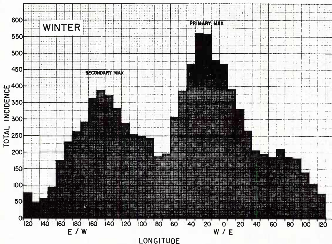
Figure 1.1. Total Incidence of Jet Stream Centurms in 10 Degree Sectors of Longitude Summed over Latitudes 50°N. - 85°N. for Winter.
