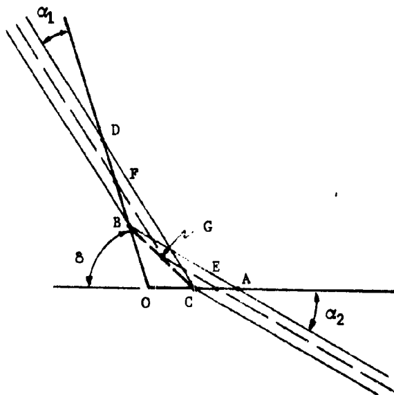
Figure 12. Geometry for in-scattering corner effect.
