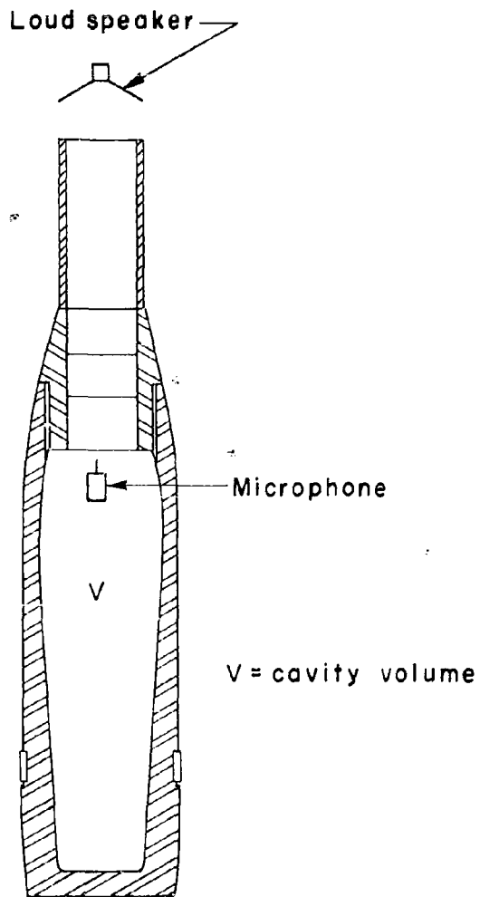
FIGURE 2. FIRST METHOD OF RESONANCE DETECTION
