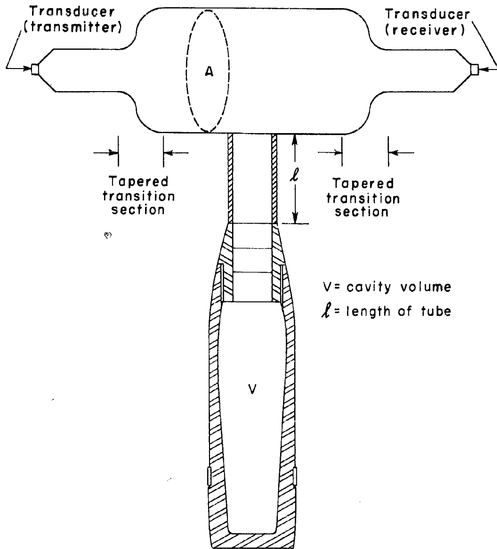
FIGURE 4. SECOND METHOD OF DETERMINING RESONANCE
