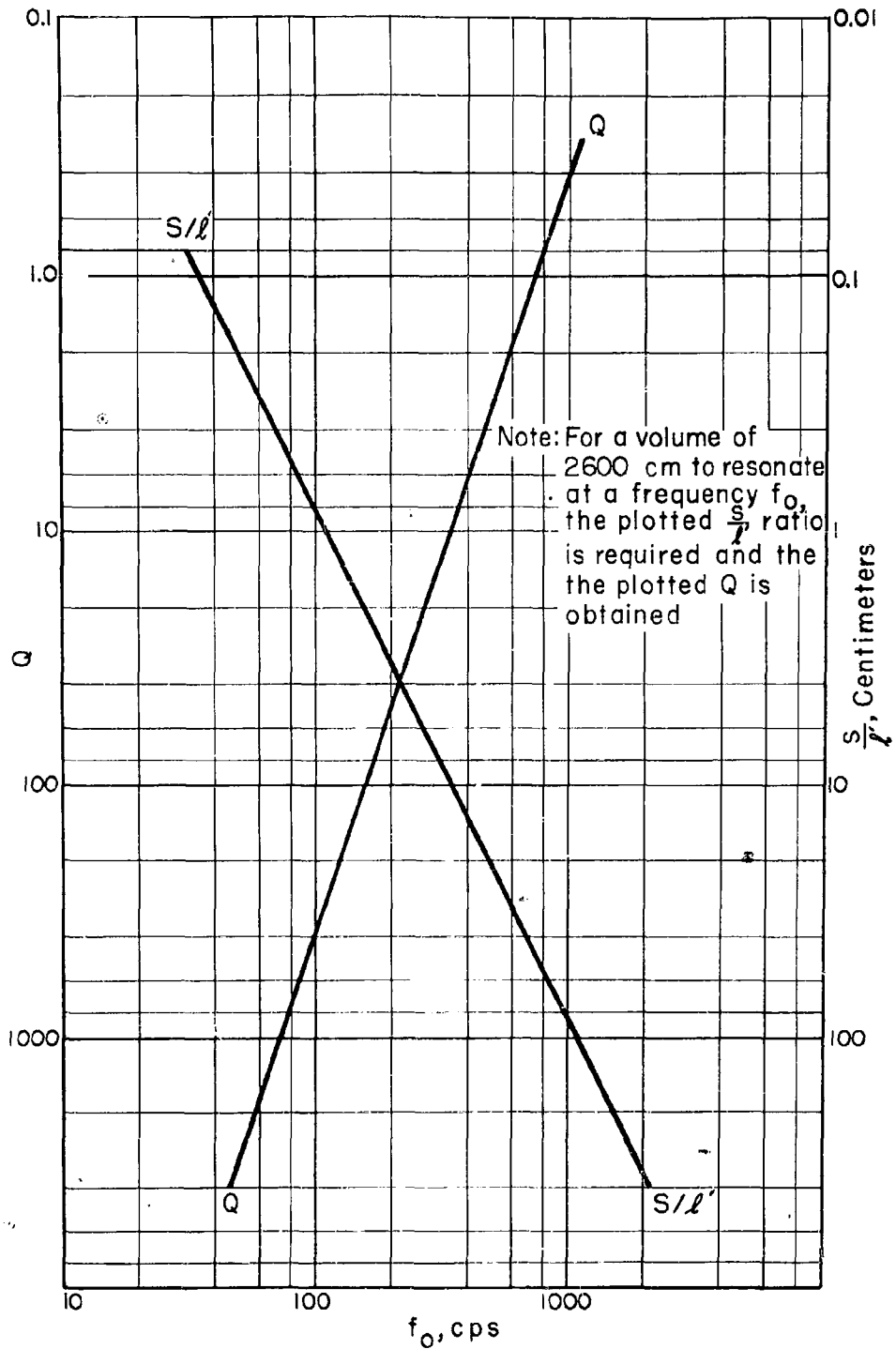
FIGURE 3. DESIGN CURVES FOR V=2600 \text{ cc}
