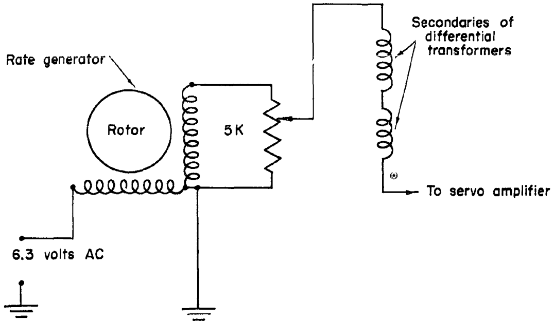
FIGURE 1. "RATE" CIRCUIT A-5166
