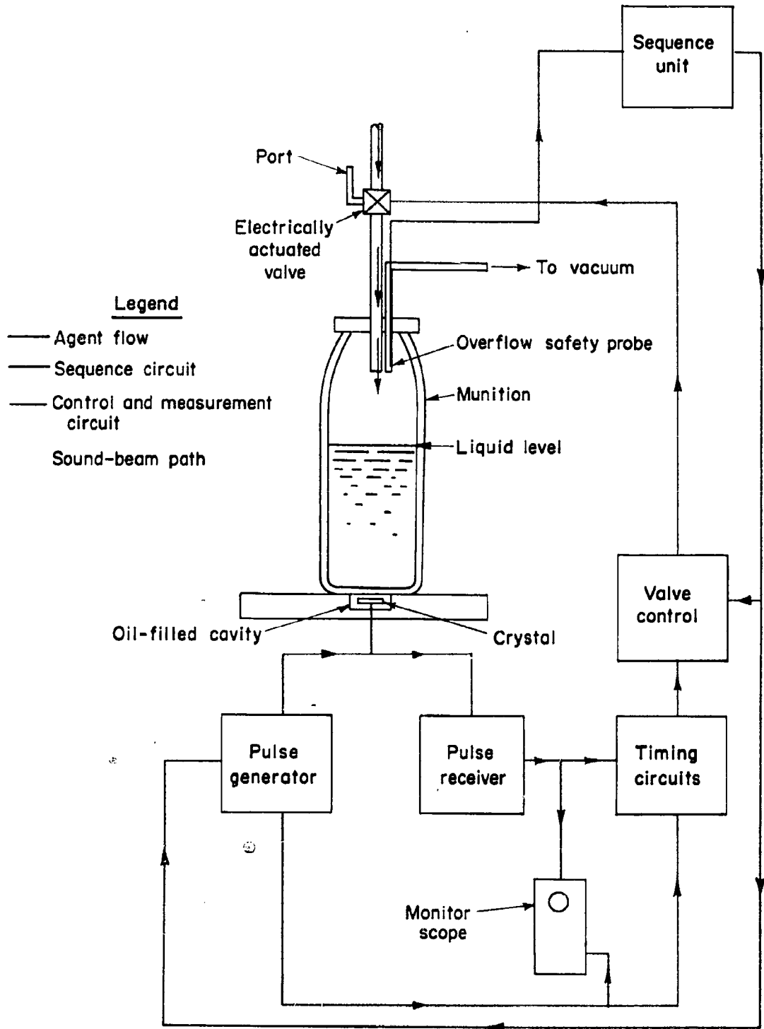
FIGURE 2. ULTRASONIC PULSE TECHNIQUE FOR LIQUID-LEVEL CONTROL
