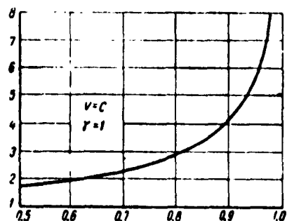
Velocity of Rocket in Fractions of the Speed of Light
