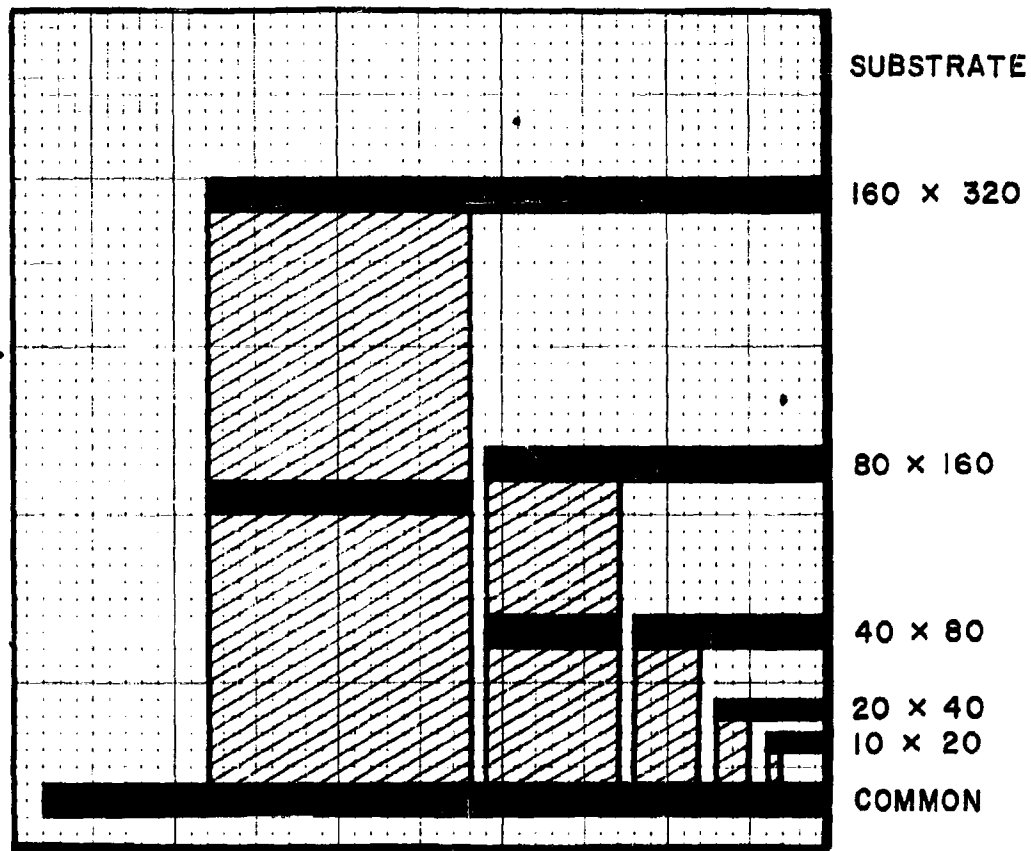
RESISTOR LAYOUT
