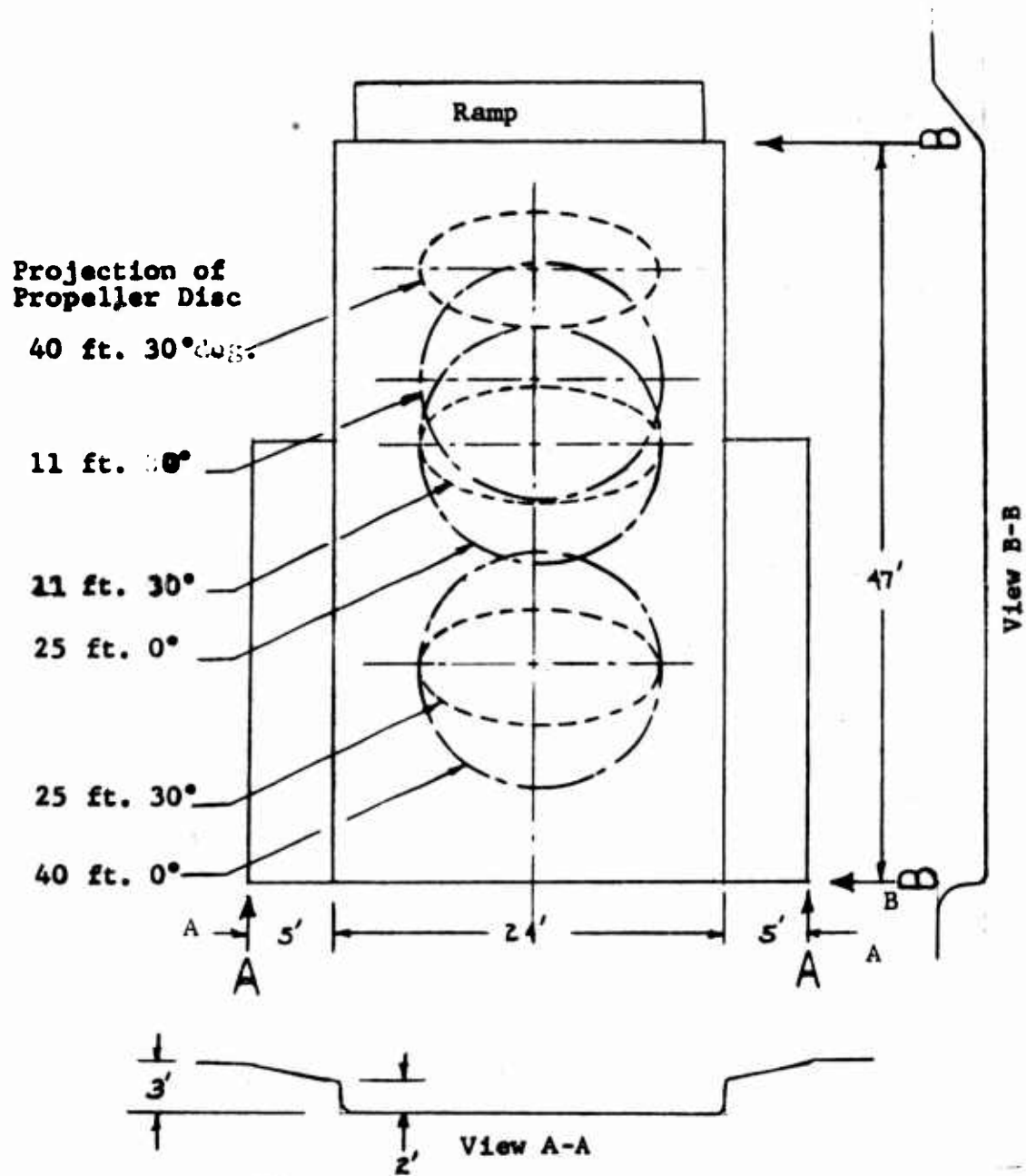
Figure 7: GEOMETRY OF WATER TEST POOL (SHOWING LOCATION OF PROJECTION OF PROPELLER DISC ALONG PROPELLER SHAFT AXIS AT THE GROUND).
