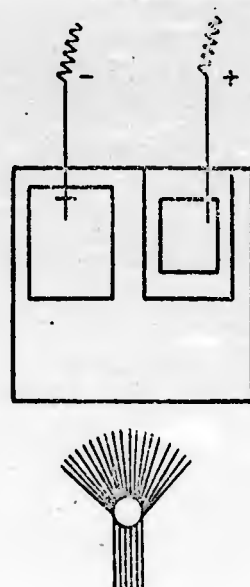
Fig. 17. Apparatus for obtaining rubidium and cesium by the electrolysis of fused salt.
