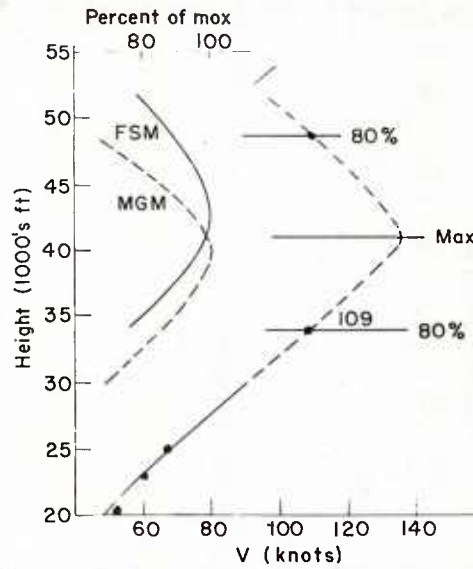
Fig. 10.10 Vertical wind profile at Jackson, Miss. (JAN), 6 March 1958, 0000 GMT. Also portions of wind profiles at FSM and MGM, expressed in per cent of the maximum wind at these stations. Extrapolated part of wind profile dashed.
