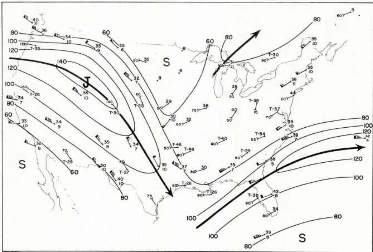
Fig. 2.14 LMW chart, 22 April 1958, 00Z.
