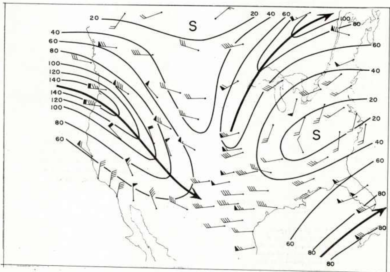
Fig. 2.10 300-mb winds, 20 April 1958, 00Z. Solid lines are jet stream axes, isobars in knots, S denotes slow areas.
