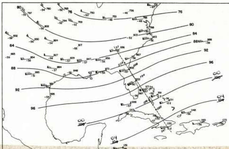
Fig. 5.7 300 mb chart 11 February 1958, 00GCT. Contours in 100's feet base 20,000 feet.
