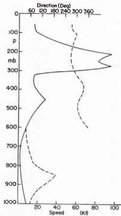
Fig. 8.16 Vertical profile of wind direction (dashed) and wind speed (solid) at San Juan, Puerto Rica, 1 April 1953, 0300 GCT. Four-minute overaged winds were used for construction of this diagram.
