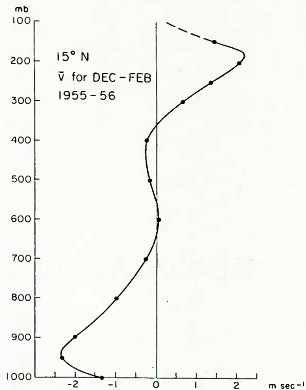
Fig. 12.6 Mean meridional wind component (m/s) for latitude 15^{\circ} N, December 1955-February 1956, as a function of pressure (Polmén, Riehl, Vuorela, 1958).
