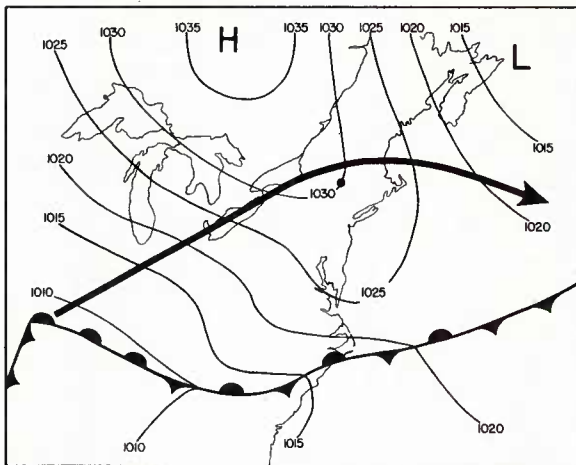
Fig. 8.14 Surface fronts and isabars, also jet stream axis, 2 March 1953. Dot marks lacotion of Schenectody.
