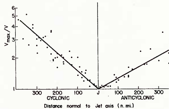
Fig. 2.8 Distribution of windspeed in layer of maximum wind normal to jet axis for strong jet streams, expressed in terms of the ratio of core speed to the speed at any station (Reiter 1958).
