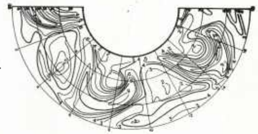
Fig. 12.36 Photograph of surface velocity field and isotochs during vortex stage of unsteady experiment. Courtesy of Dr. Dave Fultz.
