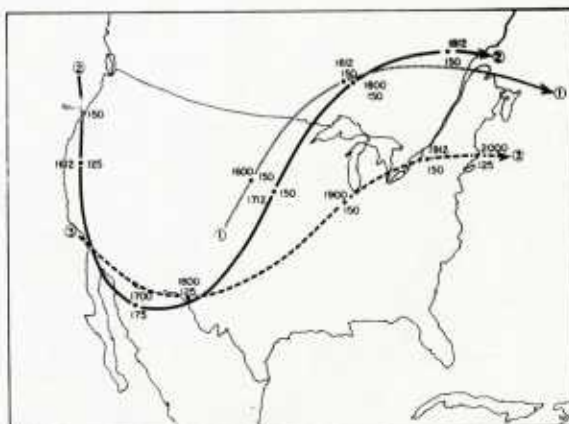
Fig. 7.6 Track of principal high-speed centers, 16-20 November 1958. Position, time and intensity (central closed isotach) given.
