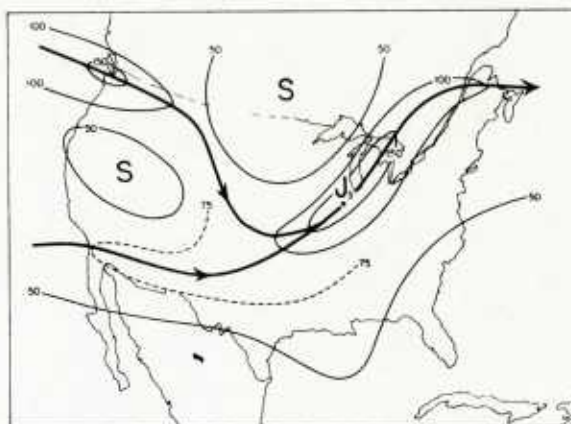
Fig. 7.4 Jet stream axes and isotachs, 19 November 1958, 00GCT.
