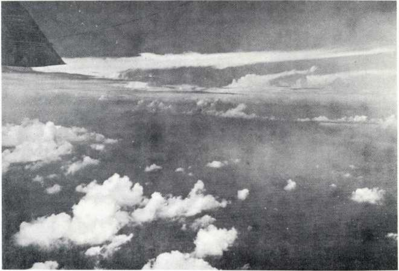
Fig. 8.17 Cumulonimbus extending into fast westerly current shown in Fig. 8.16, photographed from an altitude of 6,000 ft northeast of Puerto Rico on 1 April 1953, camera pointed toward NNE (Malkus and Ronne, 1954) Courtesy of Dr. J. S. Malkus.
