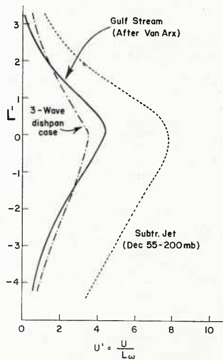
Fig. 12.7 Comparison of three jet-stream systems on a non-dimensional scale, where L is the distance from the jet axis over which the kinetic energy decreases to 50 percent of that at the core.
