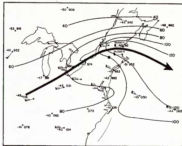
Fig. 8.15 300 mb chart, 2 March 1953, 1500 GCT. 300 mb heights in tens of feet, first digit omitted; temperatures in ^{\circ}\text{C} , isotachs in knots.
