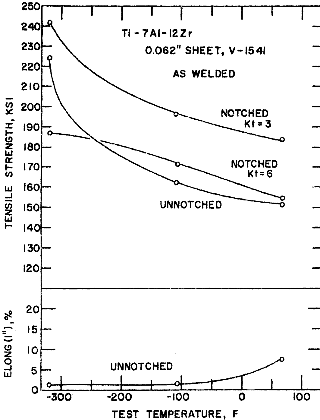
FIGURE 6 SUB-ZERO TEMPERATURE STANDARD AND NOTCH TENSILE PROPERTIES OF AS-WELDED Ti-7Al-12Zr SHEET. (V-1541, Sheet A-4802, 0.062in.)
