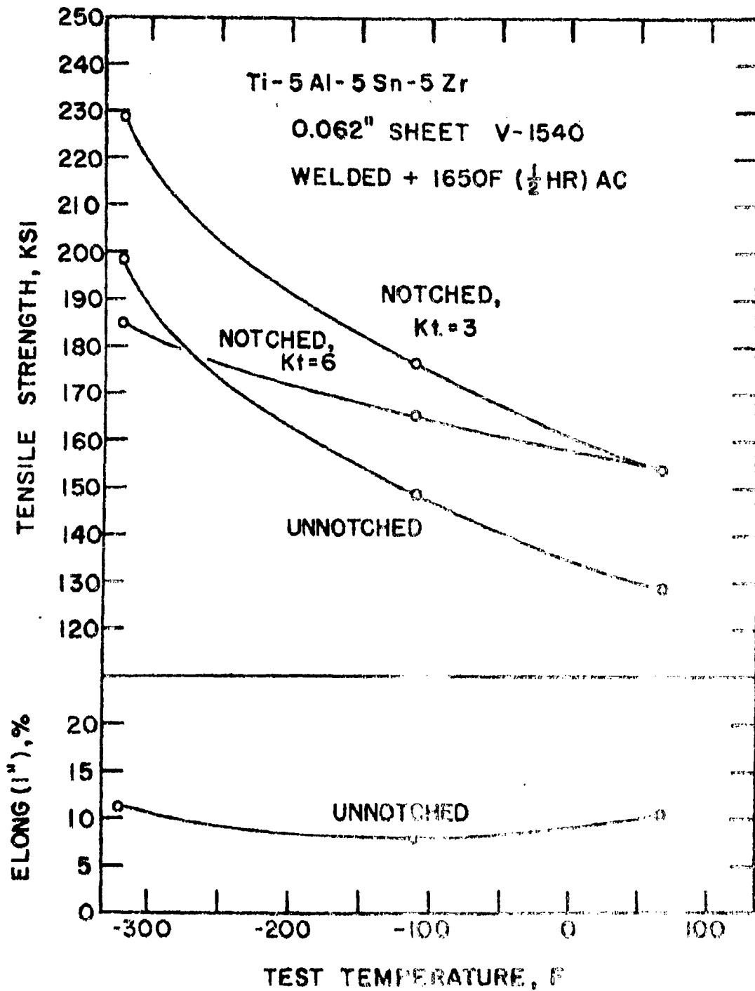
FIGURE 5 SUB-ZERO TEMPERATURE STANDARD AND NOTCH TENSILE PROPERTIES OF WELDED Ti-5Al-5Sn-5Zr SHEET, WELDED + 1650F (1/2 hr) AC. (V-1540, Sheet A-4804, 0.062in)
