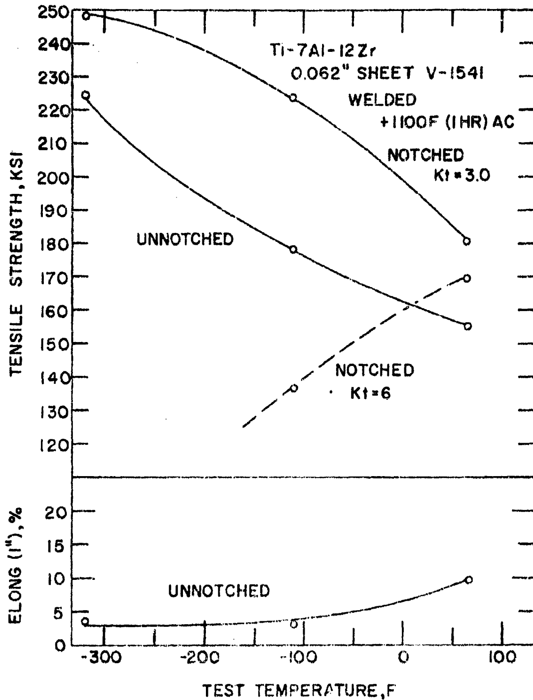
FIGURE 7 SUB-ZERO TEMPERATURE STANDARD AND NOTCH TENSILE PROPERTIES OF WELDED Ti-7Al-12Zr SHEET, WELDED + 1100F (1 hr) AC. (V-1541, Sheet A-4802, 0.062in)
