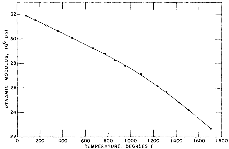
Figure 35. Dynamic Modulus as a Function of Temperature for Rene 41 (Heat Treated)
