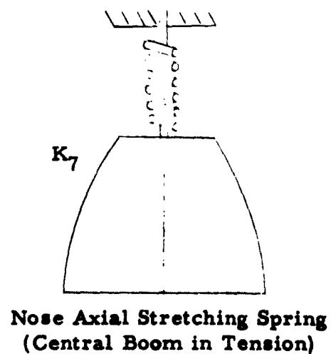
FIG. 2 - SPRING RESTRAINT SCHEME FOR BOUNDARY CONDITIONS
