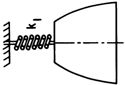
(b) NOSE AXIAL STRETCHING SPRING. (CENTRAL BOOM IN TENSION)
