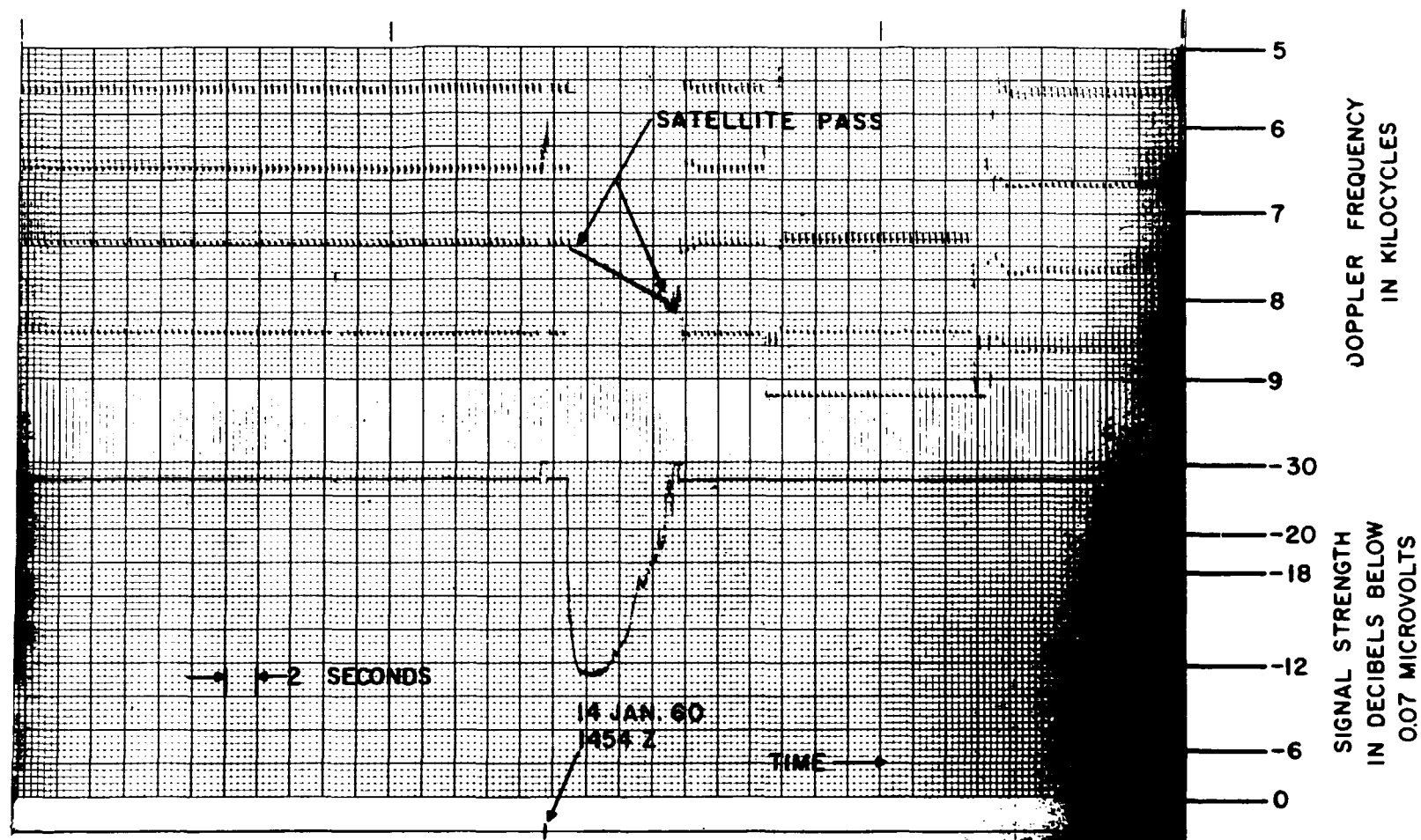
ARPA-BRL DOPLOC DOPPLER RECORD OF 58 DELTA REV. 8734, FORREST CITY, ARKANSAS MEASURED 1454:02 Z, PREDICTED 1452 Z ALTITUDE 186 MILES, 326 EAST FT. SILL CENTER ANTENNA, NORTH-SOUTH PASS
