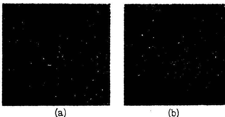
Fig. 6 Increase in pit density with deformation (a) Undeformed. (b) Deformed to approximately 0.1 per cent plastic strain. Fry's reagent with 0.2 gram \text{CuCl}_2 . (Original magnification 250X. Reduced to 50 per cent.)
