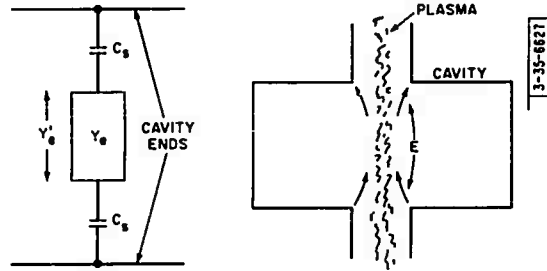
Fig. 6. Circuit with end capacitance.
